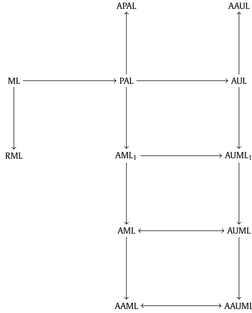
Fig. 5. The relative update expressivity of the update logics discussed in the paper. We assume transitive closure of arrows.
