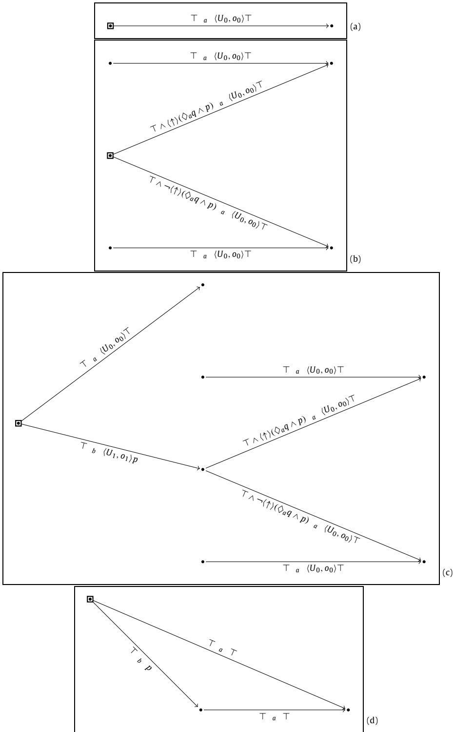
Fig. 3. Different stages in the synthesis of \Diamond_a \square_b p \wedge \Diamond_b (\Diamond_a q \vee \Diamond_a r) \wedge \square_b p .
