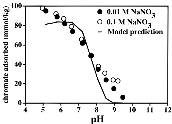
FIGURE 2. Equilibrium adsorption data for chromate adsorption on goethite versus pH. Values in legend indicate background electrolyte ( \text{NaNO}_3 ) concentrations.
