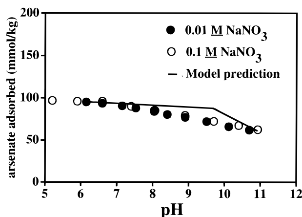
FIGURE 1. Equilibrium adsorption data for arsenate adsorption on goethite versus pH. Values in legend indicate background electrolyte (NaNO 3 ) concentrations.
