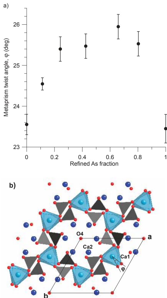
FIGURE 10. (a) Metaprisms twist angle, \phi , as a function of refined As fraction. (b) View of HAP structure looking down [0001], showing the metaprisms twist angle, \phi , which relates triangles formed by O1 and O2 atoms. Ca1 sites shown as metaprisms; Ca2 shown as spheres.
