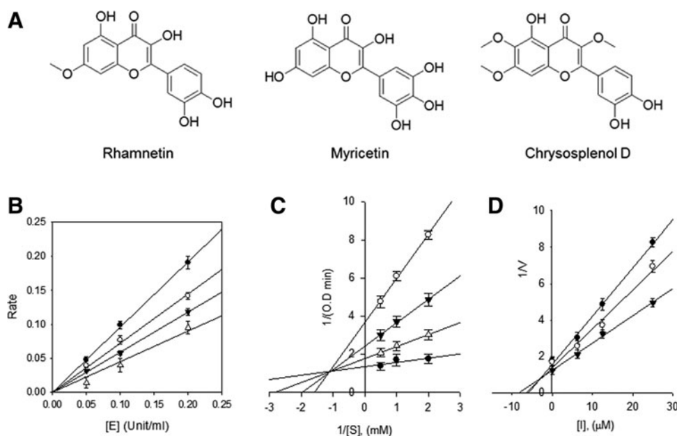
FIG. 1. (A) Chemical structure of components in AA extract: rhamnetin, myricetin, and chrysoresplenol D. (B) The catalytic activity of \alpha -glucosidase as function of enzyme concentration at different concentrations of myricetin ( \bullet , 0 \mu\text{M} ; \circ , 3.125 \mu\text{M} ; \blacktriangledown , 6.25 \mu\text{M} ; and \triangle , 12.5 \mu\text{M} ). (C) Lineweaver-Burk plot analysis of the inhibition kinetics of \alpha -glucosidase by myricetin ( \bullet , 0 \mu\text{M} ; \circ , 6.25 \mu\text{M} ; \blacktriangledown , 12.5 \mu\text{M} ; and \triangle , 25 \mu\text{M} ); conditions were as follows: 0.15 mM p-nitrophenyl- \alpha -D-glucopyranoside, 0.1 units of \alpha -glucosidase, and 50 mM potassium phosphate buffer (pH 6.8) at 37°C. (D) Dixon plot analysis of the inhibition kinetics of \alpha -glucosidase by myricetin ( \bullet , 0.5 mM; \circ , 1 mM; and \blacktriangledown , 2 mM). AA, Artemisia annua .
