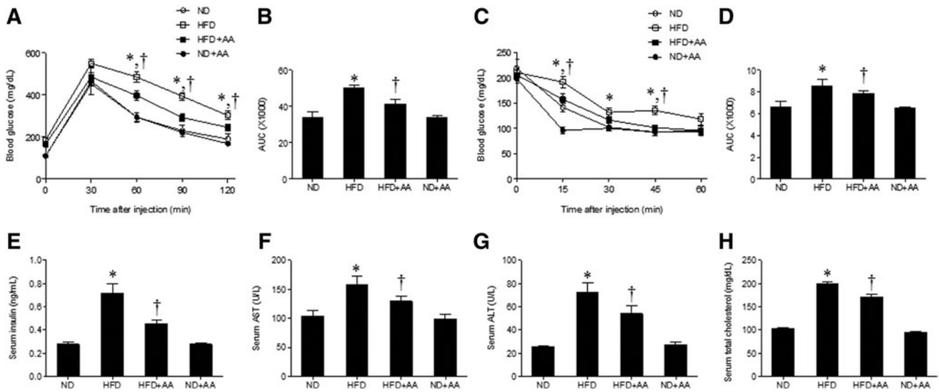
FIG. 3. Effects of AA extract on blood glucose, serum insulin, and metabolic parameters in HFD-fed mice. (A) Blood glucose levels after injection of D-glucose (2 g/kg). (B) Area under the curve (AUC) for glucose tolerance test. (C) Blood glucose levels after insulin treatment (0.75 U/kg). (D) AUC for insulin tolerance test. Serum insulin (E), aspartate aminotransferase (F), alanine aminotransferase (G), and total cholesterol (H) levels. Data ( n=6 mice per group) are presented as the mean \pm SEM. * P < .05 for ND-fed mice versus HFD-fed mice. † P < .05 for HFD-fed mice versus HFD+AA-fed mice.
