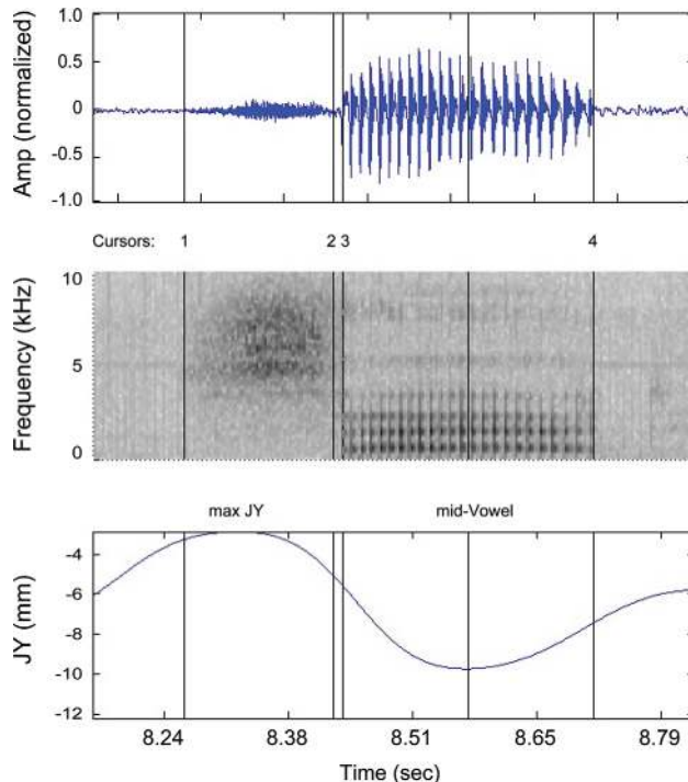
FIG. 2. (Color online) Example illustrating acoustic segmentation of sad as spoken by subject JW11. Top: Speech waveform. Middle: Spectrogram. Bottom: JY_y , the y-component of the jaw pellet. Vertical cursor lines in all three graphs indicate (1) frication onset, (2) frication offset, (3) vowel onset, and (4) vowel offset. Max-JY indicates the time at which JY_y reaches its maximum height during the [s]; Mid-vowel indicates the midpoint between vowel onset and offset.
