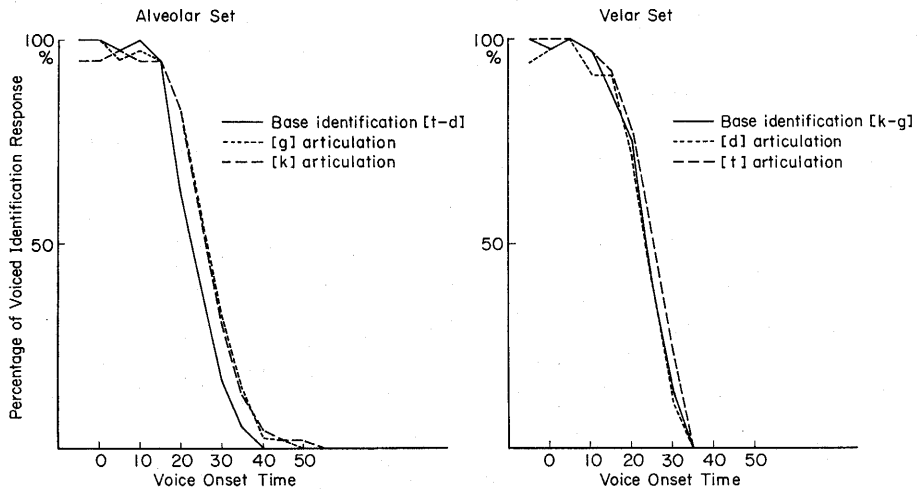
Fig. 1. Percentage of voiced identification responses [d] and [g] obtained with and without articulatory effects. The solid lines indicate the base identification functions and the dotted and dashed lines, the identification functions after repetitive articulation of voiced and voiceless consonants.
