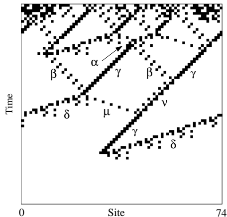
Figure 11: Filtered version of a space-time diagram of a one-dimensional, binary-state, r = 3 CA. Homogenous domains are mapped to white, domain borders to black. Domain borders can be interpreted as particles or molecules. Figure taken from [63]
