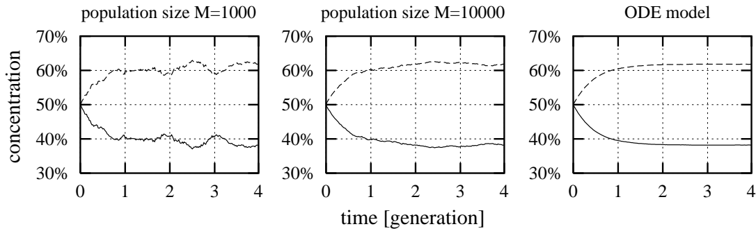
Figure 1: Comparison of the accuracy between the explicit simulation of collisions and the numerical integration. The upper curve represents the concentration of molecular species B. Left: Simulation of a population with 10^3 elements. Middle: Simulation of a population with 10^4 elements. Right: Numerical integration of the ODE-Model
