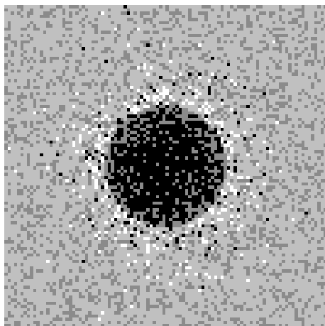
Figure 5: Stable membrane-like structure of N = 4 matrix multiplication AC with a topology. Taken from [17].
