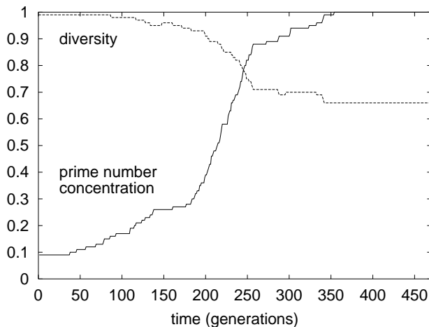
Figure 2: Development of prime number concentration and diversity. Population size M = 100 . Population initialized with number taken randomly from S = \{2, 3, \dots, 10000\}
