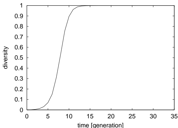
Figure 3: A simulation of the number-addition chemistry. The population is initialized with one randomly generated molecular type. The figure shows the evolution of the relative number of different string types in the population. Population size M = 10000 . Reaction s_3 = s_2 + s_1 \bmod 2^{32} .
