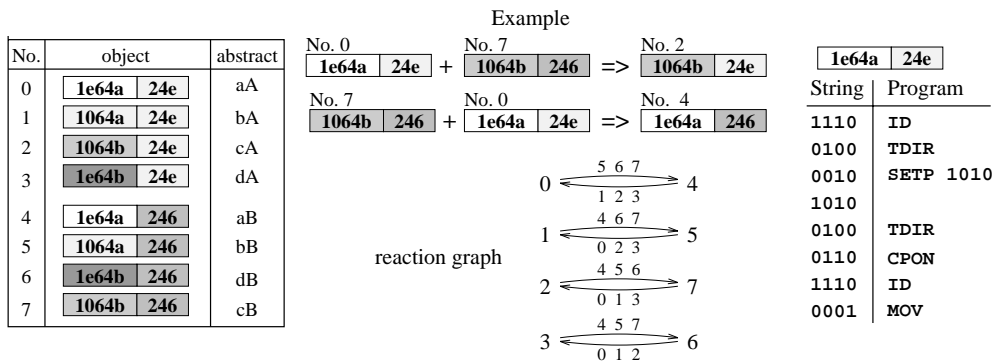
Figure 16: Example of sematic closure of a level-0 organization. Example taken from the automata reaction [40]. The self-maintaining organization consists of 8 molecular types. Their syntactic similarity allows to represent them in the form xY where x \in \{a, b, c, d\} and Y \in \{A, B\} . The semantic closure allows now to describe the interactions valid for this organization by a simple algebraic rule: xY + x'Y' \longrightarrow xY + x'Y' + x'Y .
