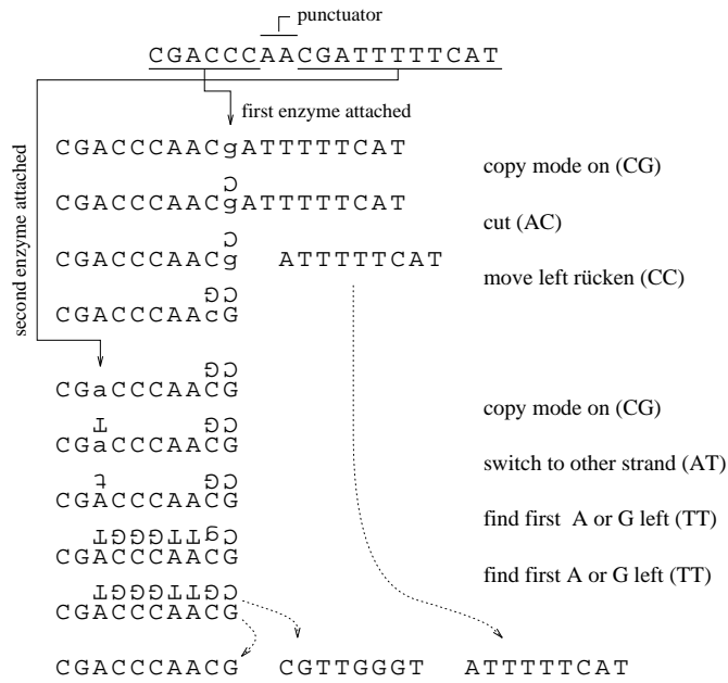
Figure 12: Example of a reaction in a Typogenetics model. Two enzymes coded by the strand CGA...AT operate on a copy of the same strand. The result are three reaction products. The current binding position of an enzyme is depicted by a lower case character. Example taken from [95].
