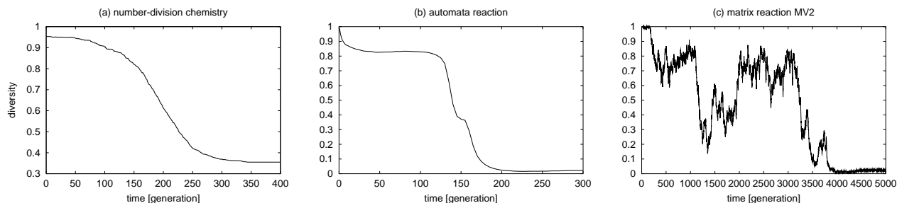
Figure 13: Examples of diversity reduction which appears in different artificial chemistries: (a) number-division chemistry (prime number chemistry), (b) automata reaction, (c) variable length matrix reaction (MV2).
