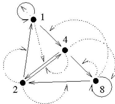
Figure 4: Reaction graph of the metabolism of N = 4 . Taken from [14].
