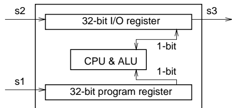
Figure 6: A schematic diagram of the automata reaction. The CPU executes the program specified by s_1 . Roughly, 4-bits are interpreted as one command. The CPU may read the program and I/O register but can only write the I/O register. With an appropriate program the contents of the program register can be copied to the I/O register.
