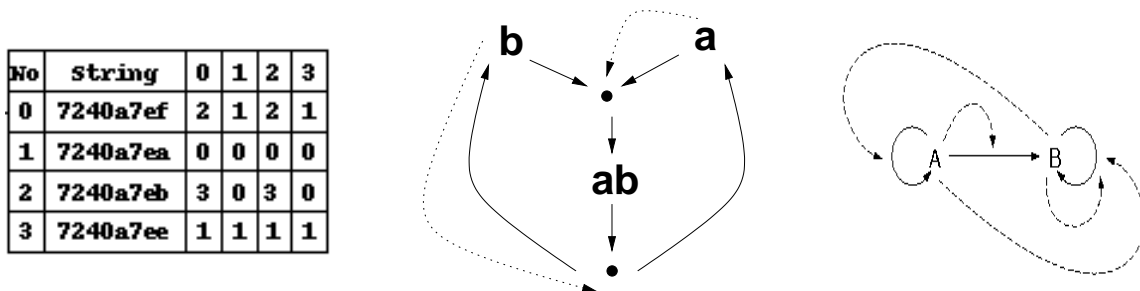
Figure 14: Left: Stable network of binary strings with reaction matrix. Middle: Network of polymer reactions. Dotted lines indicate catalytic activity. Right: Simplest stable network of \lambda -expressions. A = \lambda s_1 \cdot (s_1)\lambda s_2 \cdot \lambda s_3 \cdot (s_3)\lambda s_4 \cdot \lambda s_5 \cdot (s_5)s_4 , B = \lambda s_1 \cdot (s_1)\lambda s_2 \cdot \lambda s_3 \cdot (s_3)s_2 .
