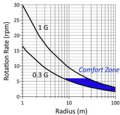
FIGURE 2 | Hypothetical comfort zone bounded by values of artificial gravity level and rotation rate based on theoretical studies in the 1960s (see Hall, 2009, for details). The “comfort zone” is the area in blue delimited by a maximum rotation rate of 6 rpm. According to the model of Stone and Letko (1965) the Coriolis and cross-coupled angular accelerations generated at these rotation rates during walking, climbing and handling materials should be the most comfortable for the crewmembers. However, very little experimental data were actually collected to validate this model. Recent data indicate that the limit of 6 rpm is overly conservative.
