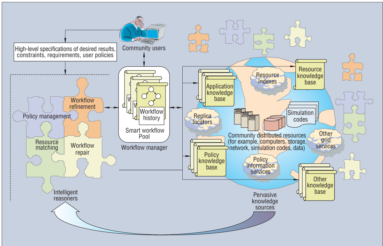
Figure 1. Distributed grid workflow reasoning.
