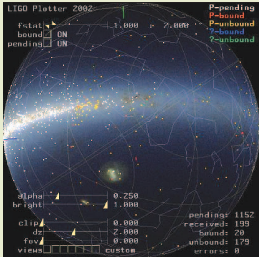
Figure A. Visualization of a Laser Interferometer Gravitational-Wave Observatory pulsar search. The sphere depicts the map of the sky. The points indicate the locations where the search was conducted. The color of the points indicates the range to which particular results belong.
