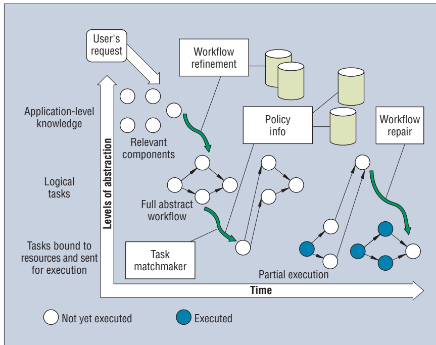
Figure 2. Workflows are incrementally refined over time by distributed reasoners.
