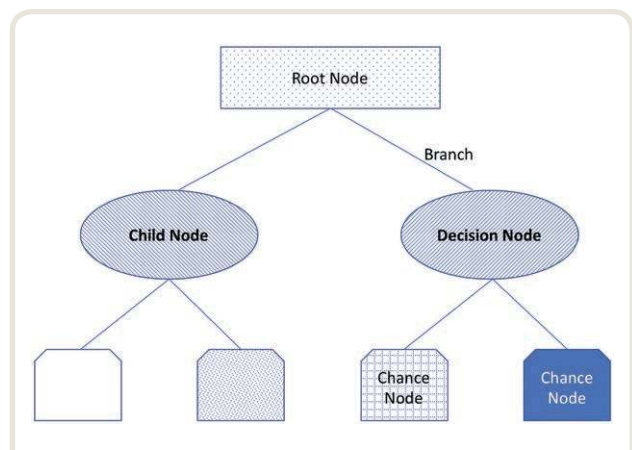
Fig. 2. An illustrative example of a decision node. Several terminologies can be used to describe decision trees. The root node is the start of the tree, and branches connect nodes. A child node is any node that has been split from a previous node, whereas a decision node is any node that allows two or more options to follow it. A chance node is any node that may represent uncertainty.
