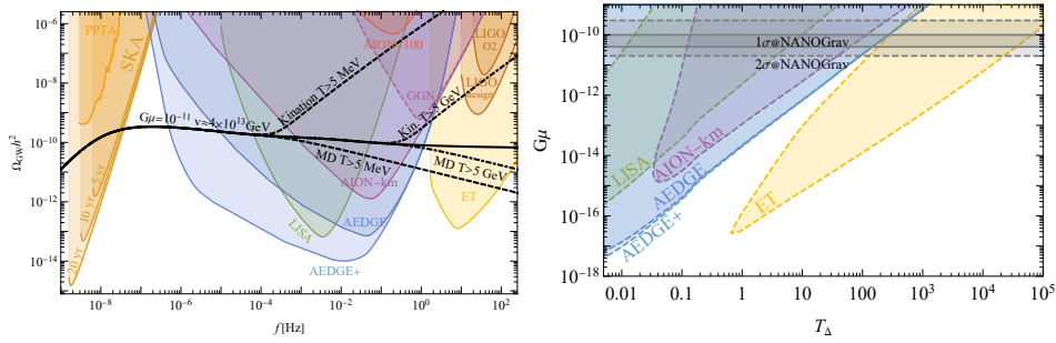
Figure 9. Sensitivities of cosmic string measurements to modifications of the cosmological expansion rate. Left panel: Kination or matter dominance (MD) at temperatures T > 5 MeV or 5 GeV. Right panel: Sensitivity to modification of the expansion rate at a temperature T_\Delta for a given value of the string tension G\mu .
