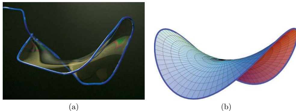
Fig. 1.1 (a) Soap film surface. (b) Mathematical model—is it correct?
