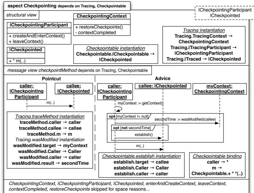
Figure 10: The Checkpointing Aspect Model
