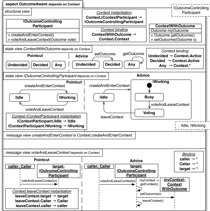
Figure 9: The OutcomeAware Aspect Model
