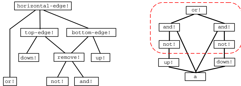
Figure 1: Two different diagrams of the un-optimized horizontal-edge! filter. On the left is the functional decomposition, which aligns so directly with the domain model. On the right is a data flow diagram, in which the boxes are the primitive filters and the edges are the data flows between them at runtime. The box labeled a at the bottom is the input image.
