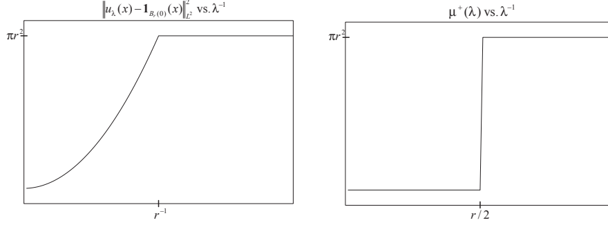
FIG. 3.1. Left: Plot of \|u_\lambda(x) - f(x)\|_{L^2}^2 vs. \lambda^{-1} for the example of Section 3, where u_\lambda(x) denotes the unique minimizer of E_2(\cdot, \lambda) . Right: Plot of \mu^+(\lambda) vs. \lambda^{-1} for the ROF model with L^1 fidelity, using the example of Section 3.
