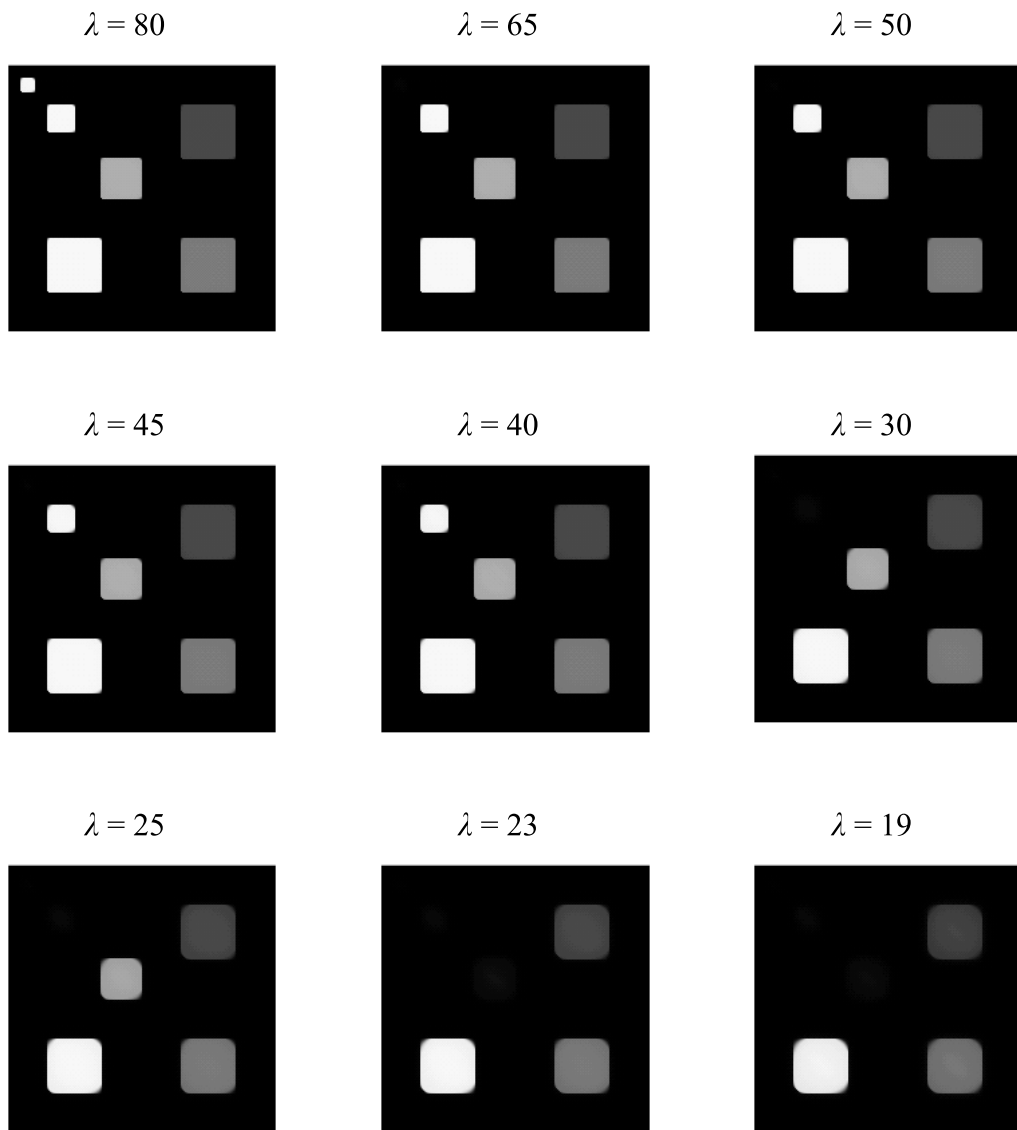
FIG. 8.2. Example of scale space generated by the total variation model with L^1 fidelity. Compare with Figure 2.
