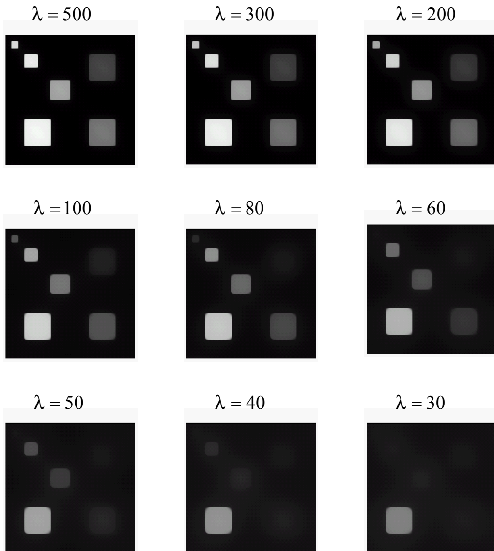
FIG. 8.1. Example of scale space generated by the standard total variation model. Compare with the same example for the model with L^1 fidelity, shown in Figure 3.
