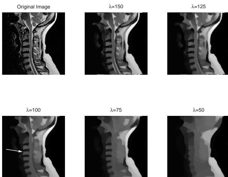
FIG. 8.5. Scale space generated by the ROF model with L^1 fidelity term.
