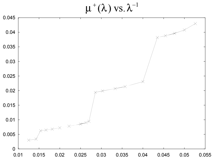
FIG. 8.3. Plot of fidelity of minimizer (i.e. \|u_\lambda(x) - f(x)\|_{L^2}^2 ) vs. \lambda^{-1} for the standard ROF model (top graph) and the plot of fidelity of minimizer (i.e. \|u_\lambda(x) - f(x)\|_{L^1} ) vs. \lambda^{-1} for the ROF model with L^1 fidelity (bottom graph).
