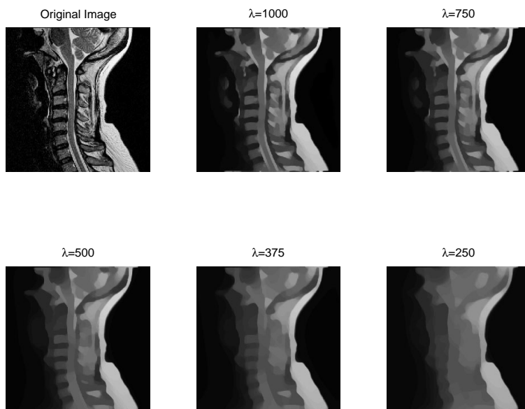
FIG. 8.4. Scale space generated by the standard ROF model.
