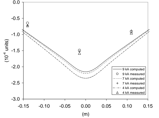
Fig. 8. Integrated b_6 ( 10^{-4} units) at R_{ref} = 10 mm along a 250 mm probe as a function of the relative position (m) of the probe center with respect to the magnet center: meas. (markers) and computations (curves).
