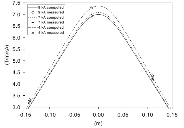
Fig. 7. Integrated transfer function (T/m/kA) at R_{ref} = 10 mm along a 250 mm probe as a function of the relative position (m) of the probe center with respect to the magnet center: meas. (markers) and computations (curves).
