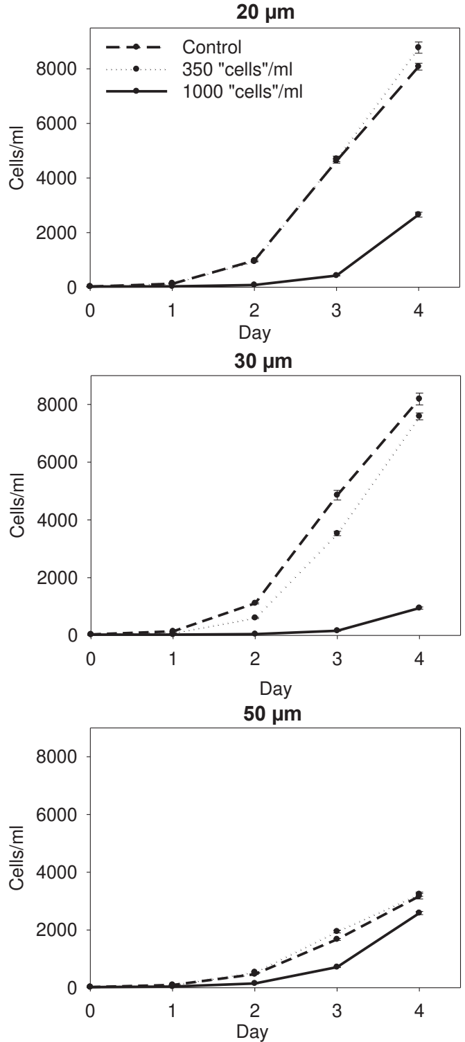
Figure 2.7 Cell concentrations as a function of time for Thalassiosira cultures of different cell sizes in two concentrations of A. fundyense filtrate. Data points are the average of number of cells/ml on each day in replicate experiments. Error bars represent the propagated SE of triplicate cell counts for each daily sample.
