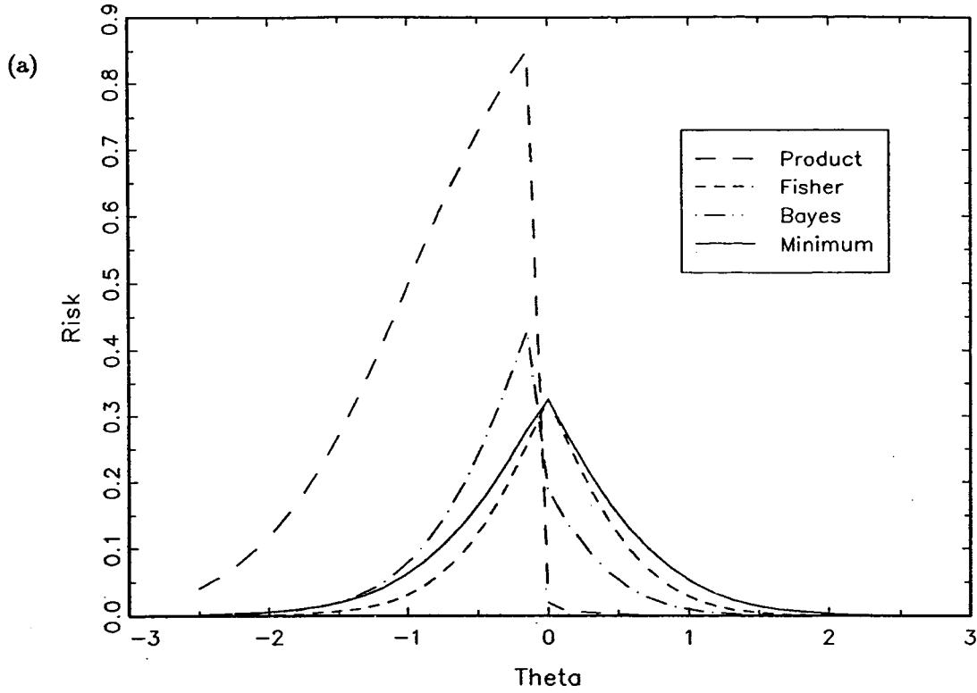
Figure 1: Simulated risks of the Fisher statistic (Product), the Fisher p-value (Fisher), the impartial Bayes rule \phi_{\mathbb{L}}(\mathbf{x}) (Bayes) and Tippett p-value (Minimum) for a normal distribution and one-sided hypothesis H_0 : \theta_i \leq 0, i = 1, 2, 3, 4 . The true parameter values have the form (\theta, \theta, \theta, \theta) for (a) and (0, 0, \theta, \theta) for (b). The x-axes of the plots represent the values of \theta .
