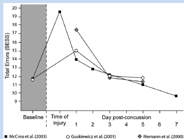
Figure 1. Mean Balance Error Scoring System (BESS) error score at baseline and following concussion.
