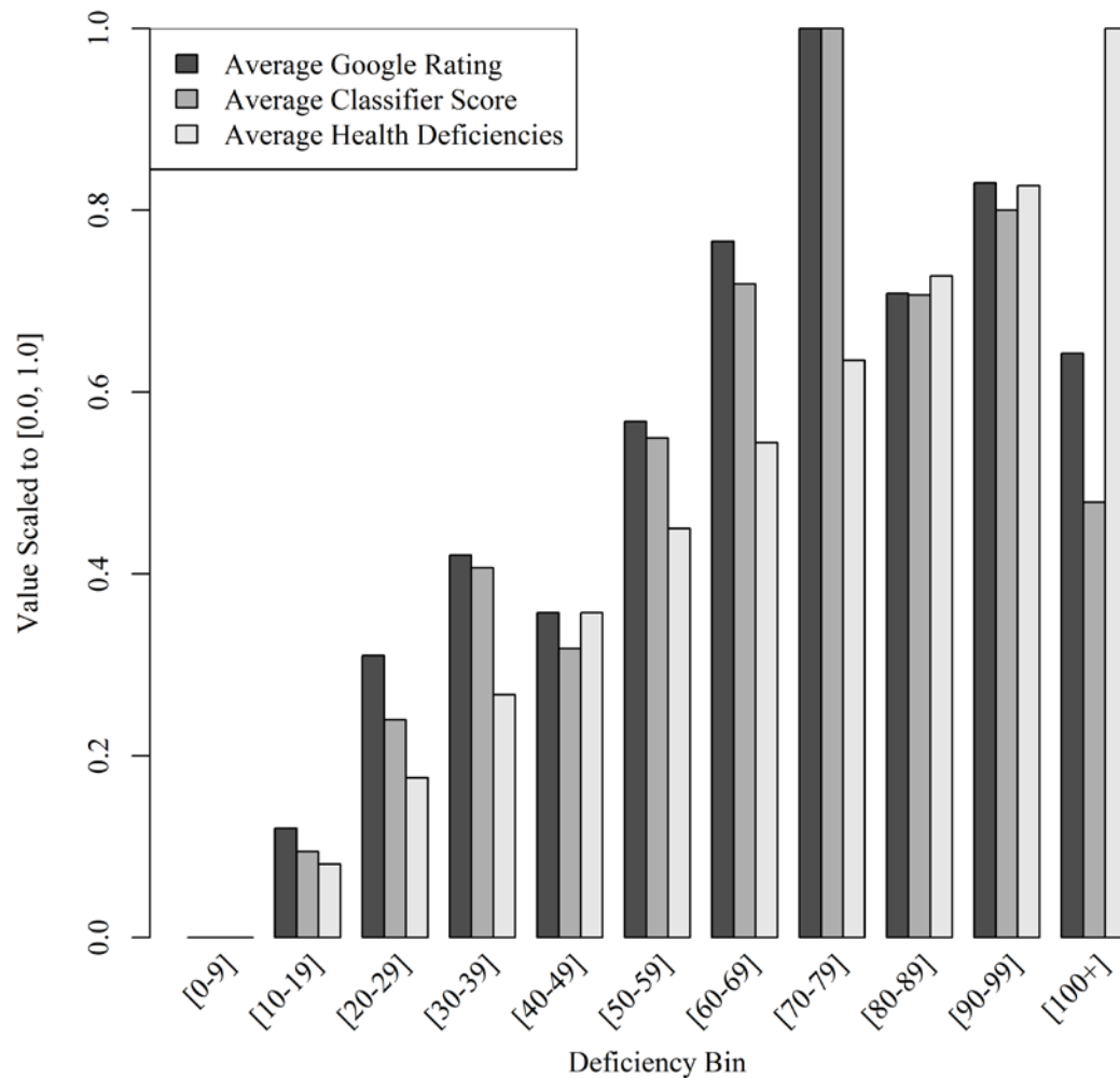
Figure 5: Illustration of correlations between average Google ratings, average classifier scores, and average health deficiency counts for providers in each health deficiency bin. The relationships between the averages remains stable across deficiency bins except for the [100+] bin, which contains only six providers.
