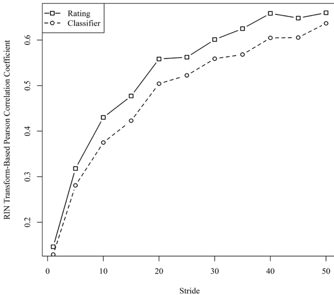
Figure 4: RIN transform-based Pearson correlation coefficients between Google ratings or classifier scores and CMS health deficiency counts as a function of stride. The stride is the number of providers with similar deficiency counts merged to produce an aggregated provider with an effectively larger number of reviews. Aggregating providers enables extrapolating the potential correlation coefficients achievable with more reviews per provider without generating synthetic reviews. Google ratings correlate better with health deficiency counts, while classifier scores correlate nearly as well, even though the classifier scores reflect references to elder abuse rather than overall quality of care.
