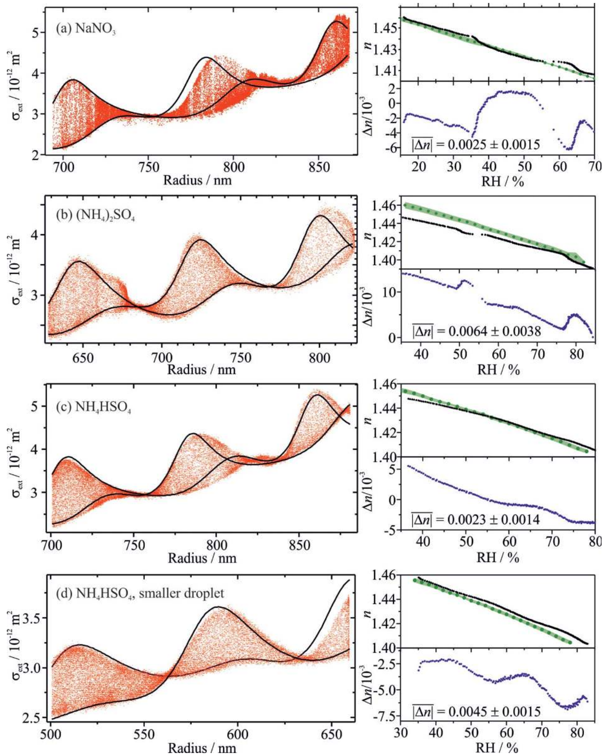
Figure 7. The best-fit CSW Mie envelopes (lines, black) to experimentally measured \sigma_{ext} data (points, red) for fine mode particles containing the hygroscopic inorganic solutes \text{NaNO}_3 , (\text{NH}_4)_2\text{SO}_4 or \text{NH}_4\text{HSO}_4 . Shown alongside each data set are the corresponding variation in the best-fit RI, n_{finer} (points, black) compared against the determined RI variation from measurements on coarse mode particles, n_{coarser} (points, green, with error envelope where the envelope represents one standard deviation in measurements over several droplets). The points (blue) in the plot of residuals represent \Delta n = n_{coarse} - n_{finer} with the magnitude and standard deviation in |\overline{\Delta n}| quoted.
