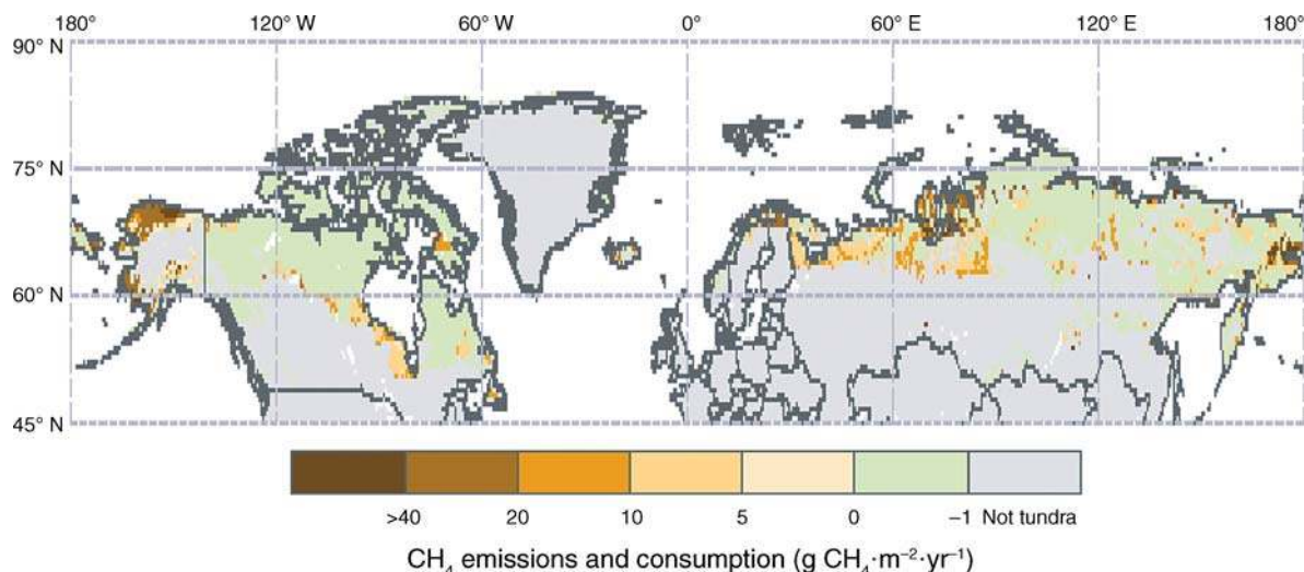
FIG. 7. Simulated net \text{CH}_4 emissions and consumption in tundra ecosystems in the pan-Arctic region ( 45^\circ \text{N} and above) during the 1990s. Positive values indicate the net \text{CH}_4 release to the atmosphere, and negative values indicate the \text{CH}_4 uptake from the atmosphere.
