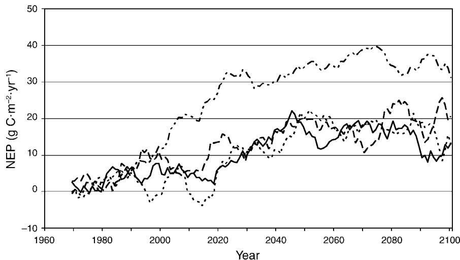
FIG. 5. Ten-year mean of future Arctic net ecosystem production (NEP) simulated by LPJ using climatologies from GFDL (dashed line), HadCM3 (solid line), CCC (dotted dashed line), and ECHAM3 (dotted line; see Table 2 for abbreviation explanations) for the emission scenario B2 of the Special Report on Emission Scenarios (SRES; see Callaghan et al. [2004, 2005] for circumpolar maps).
