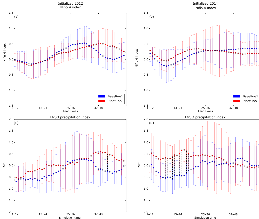
Figure 10. Top row shows the Niño 4 index and bottom row shows the ENSO precipitation index (ESPI) for the first four prediction years calculated as a 12-month running mean to reduce variance. Left (right) column shows the 2012 (2014) initialized experiments. Error bars show the SD of the ensemble and vertical black lines indicate a significant difference.
