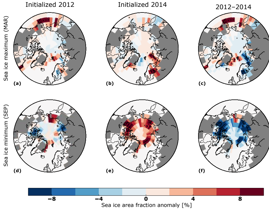
Figure 5. Differences in ensemble mean forecasts of SIC for prediction years 1–4, (a–c) for the 4-year mean maximum in March, and (d–f) for the 4-year mean minimum in September. (a, d) Exp-2012 (Pinatubo-2012 – b1-2012), (b, e) exp-2014 (Pinatubo-2014 – b1-2014), and (c, f) the difference between the two (exp-2012 – exp-2014). Crosses denote values significantly different from zero exceeding a 5 % level.
