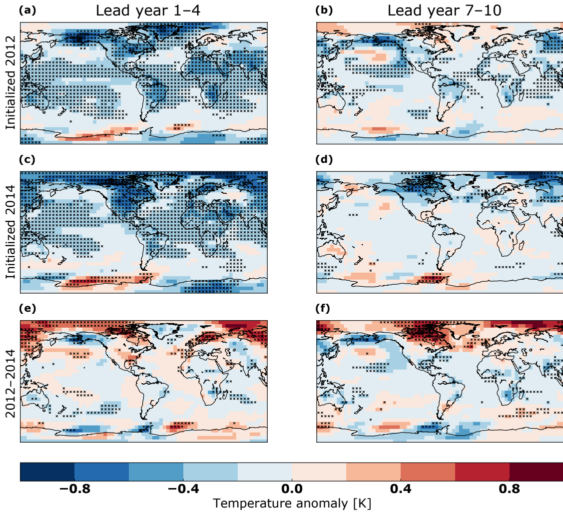
Figure 3. Differences in ensemble mean forecasts of TAS for prediction years 1–4 ( a, c, e ) and 7–10 ( b, d, f ). Top row ( a, b ) shows exp-2012 (Pinatubo-2012 – b1-2012), middle row ( c, d ) shows exp-2014 (Pinatubo-2014 – b1-2014), and bottom row ( e, f ) shows the difference between the two upper (exp-2012 – exp-2014). Crosses denote values significantly different from zero exceeding a 5 % level.
