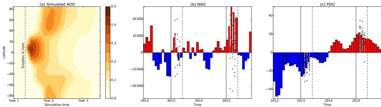
Figure 1. (a) Temporal evolution of the stratospheric aerosol optical depth (AOD) used for our simulations with a Pinatubo-like eruption. The climate indices NAO (b) and PDO (c) calculated from the assimilation model run. Lighter colors are the indices of the prediction system ensemble mean before the Pinatubo-like eruption and grey circles are the individual ensemble members. Vertical lines indicate the initialization time of our forecast experiments and vertical hatched lines indicate the start of the Pinatubo-like eruption.
