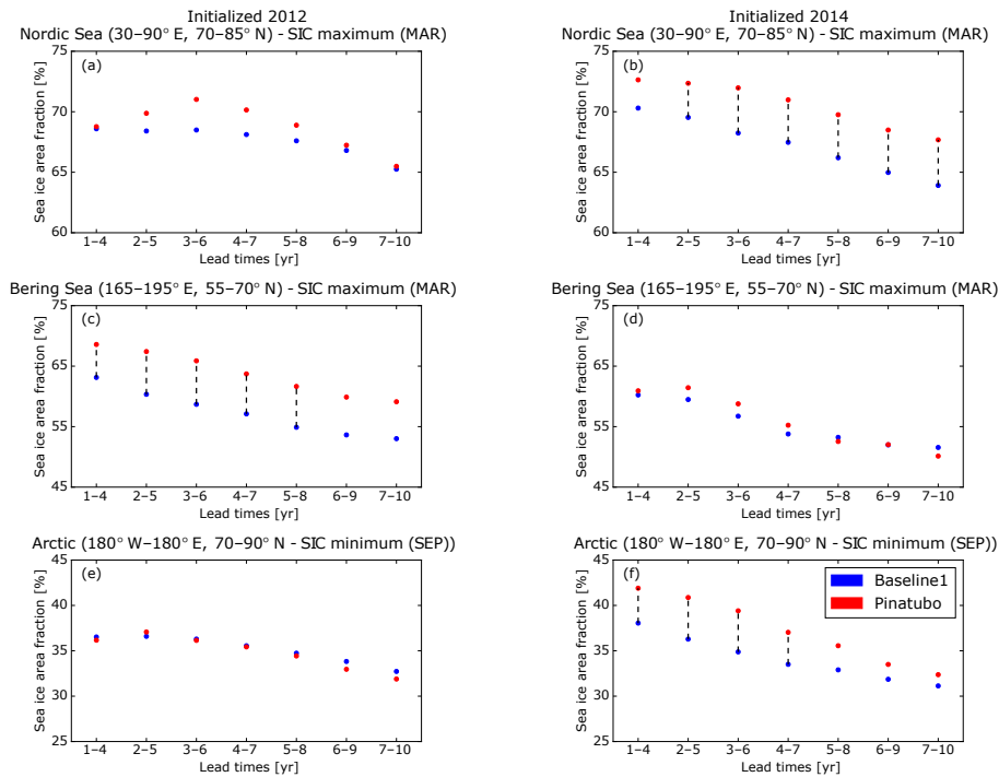
Figure 6. Same as Fig. 2, but for sea ice area fraction (SIC) maximum and minimum and different regions. (a, b) Nordic Sea (30–90° E, 70–85° N), (c, d) Bering Sea (165–195° E, 55–70° N), and (e, f) the Arctic (180° W–180° E, 70–90° N). Dashed lines indicate significant differences between the values at the 5 % level.
