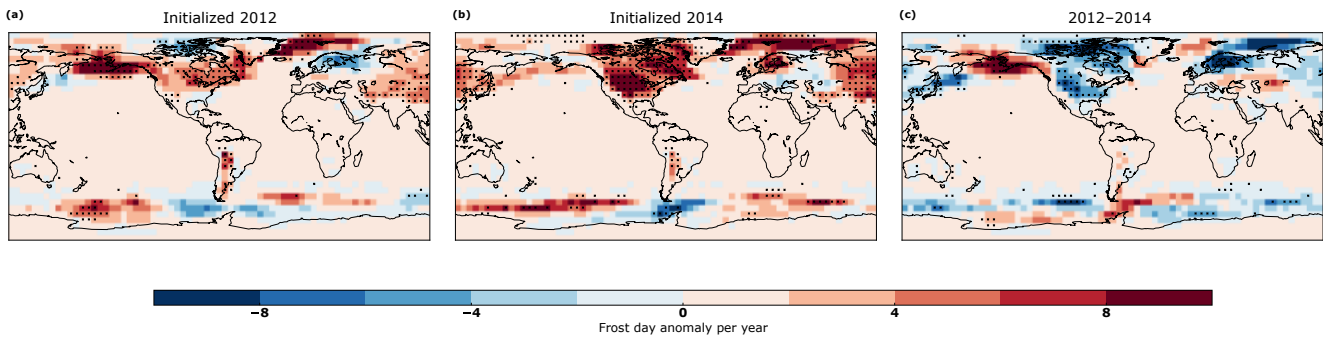
Figure 7. Differences in ensemble mean forecasts of frost days (FDs) for prediction years 1–4. (a) Exp-2012 (Pinatubo-2012 – b1-2012), (b) exp-2014 (Pinatubo-2014 – b1-2014), and (c) the difference between the two (exp-2012 – exp-2014). Crosses denote values significantly different from zero exceeding a 5 % level.
