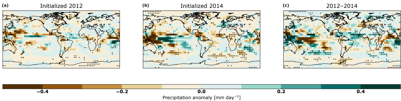
Figure 9. Same as Fig. 7, but for precipitation (PR) anomalies.
