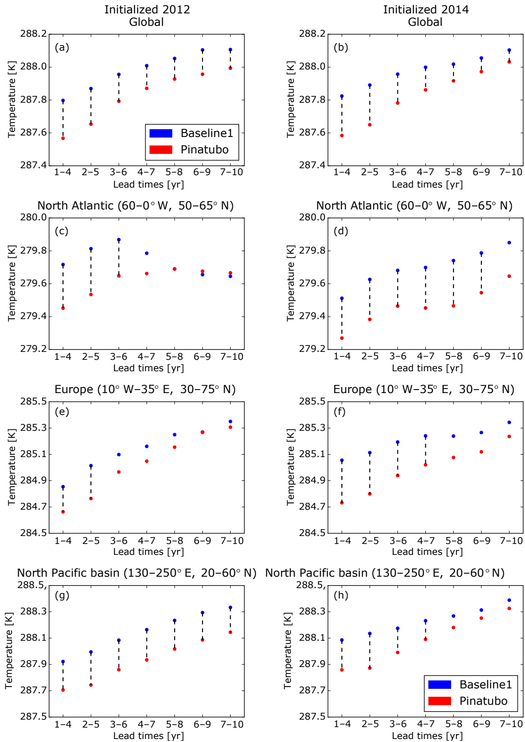
Figure 2. Time series of 4-year running mean ensemble forecast of near-surface air temperature (TAS) anomalies. The blue shows values without volcanic eruption, and red with a Pinatubo-like eruption. (a, c, e, g) Experiments initialized in 2012 and (b, d, f, h) those initialized in 2014. (a, b) Global mean, (c, d) North Atlantic ( 60^{\circ} W– 0^{\circ} E, 50 – 65^{\circ} N), (e, f) Europe ( 10^{\circ} W– 35^{\circ} E, 30 – 75^{\circ} N), and (g, h) North Pacific basin ( 130 – 250^{\circ} E, 20 – 60^{\circ} N). Dashed lines indicate significant differences between the values at the 5% level.
