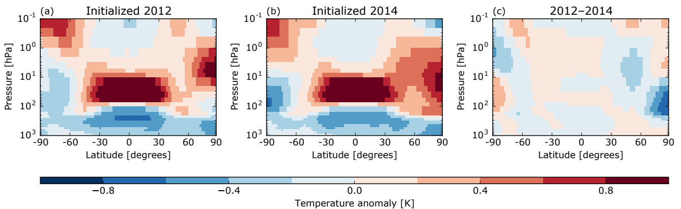
Figure 4. Differences in ensemble mean forecasts of zonal mean air temperature (TA) for prediction years 1–4. ( a ) Exp-2012 (Pinatubo-2012 – b1-2012), ( b ) exp-2014 (Pinatubo-2014 – b1-2014), and ( c ) the difference between the two (exp-2012 – exp-2014).
