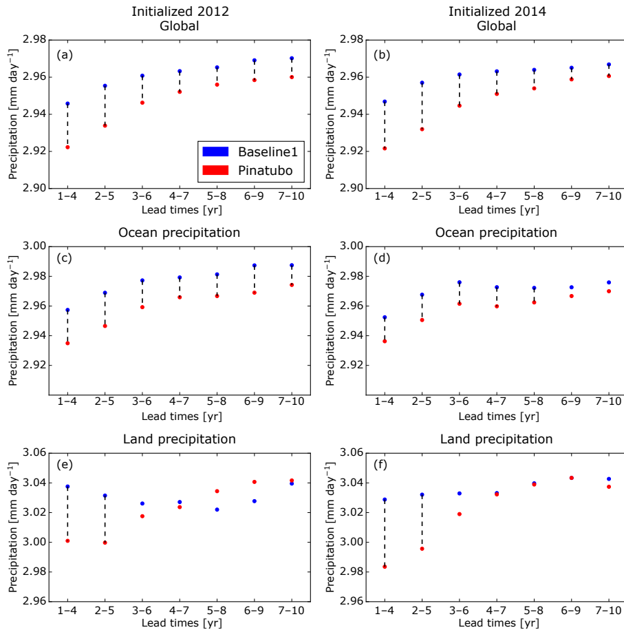
Figure 8. Same as Fig. 2, but for precipitation (PR) and different regions. (a, b) Global mean, (c, d) ocean only, and (e, f) land only. Dashed lines indicate significant differences between the values at the 5% level.
