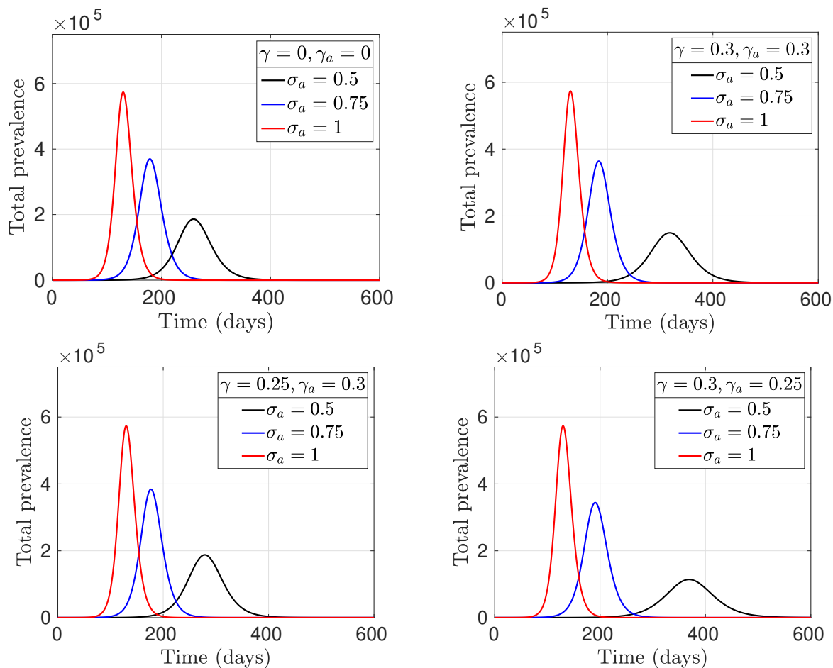
Figure 3: Effect of adherence to NPIs on COVID-19 epidemic. The total disease prevalence over time for different values of the parameter \sigma_a (used to model reduction in virus shedding, susceptibility, and onward disease transmission for the adherent population) and the movement rates \gamma (non-adherence to adherence) and \gamma_a (adherence to non-adherence). Top left: \gamma = \gamma_a = 0 with \tilde{f} = 0.5 , top right panel: \gamma = \gamma_a = 0.3 , bottom left: \gamma = 0.25 and \gamma_a = 0.3 , and bottom right: \gamma = 0.3 and \gamma_a = 0.25 . All other parameters are as given in Table 2 with initial conditions S(0) = (1 - f)N, E(0) = 0, I(0) = 1, R(0) = 0, S_a(0) = fN, E_a(0) = 0, I_a(0) = 1, R_a(0) = 0 and V(0) = 1 .
