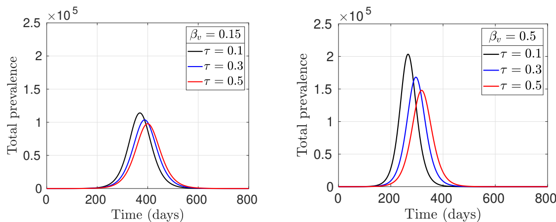
Figure 7: Effect of environment cleaning/sanitization on disease dynamics. Total disease prevalence over time for different environment cleaning/sanitization rate \tau and the indirect transmission rate \beta_v for non-adherent population. Left panel: \beta_v = 0.15 and right panel: \beta_v = 0.5 . \tau = 0.1 (black), \tau = 0.3 (blue), and \tau = 0.5 (red). All other parameters are as given in Table 2 and initial conditions are the same as in Figure 3.
