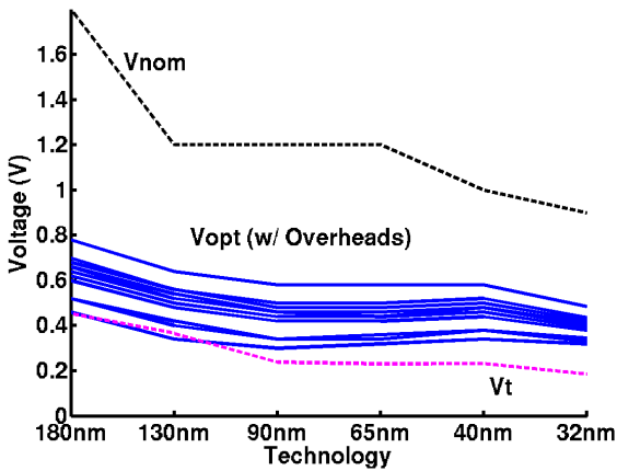
Figure 7: V_{opt} across technologies when including all three overheads. V_{opt} has been trending downward with each generation and is \sim 200\text{-}400\text{mV} above V_t for most benchmarks.
