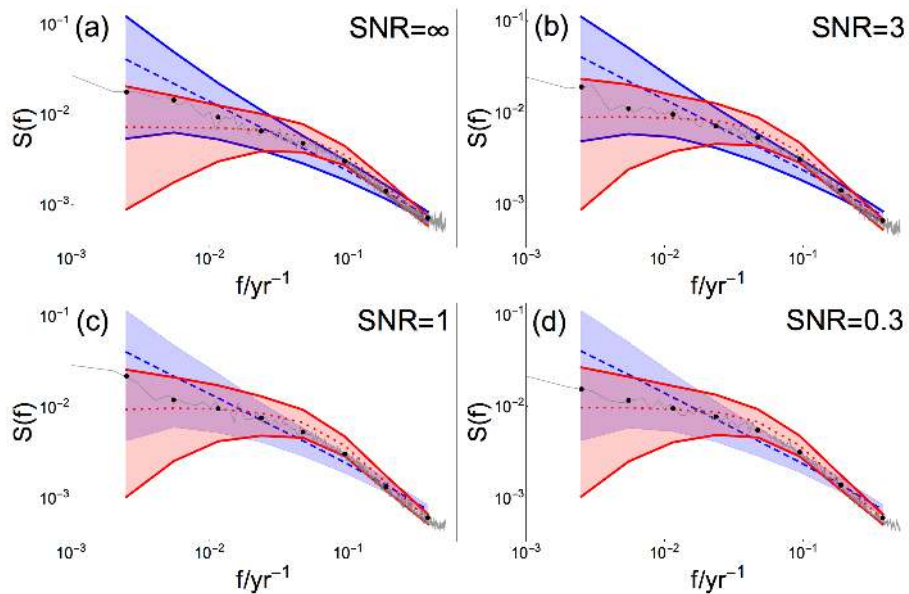
Figure 4. Mean raw and log-binned PSD for local reconstructed data at a site between proxies (gray curve and dots, respectively) generated from \beta_{\text{target}} = 0.75 and different SNR indicated in (a)–(d). Colored shading and dashed/dotted lines indicate 95 % confidence range and the ensemble mean, respectively, for a Monte Carlo ensemble of fGn with \beta = 0.75 (blue) and of AR(1) processes with \alpha estimated from BARCAST (red). The confidence ranges found consistent with the data are drawn with solid lines.
