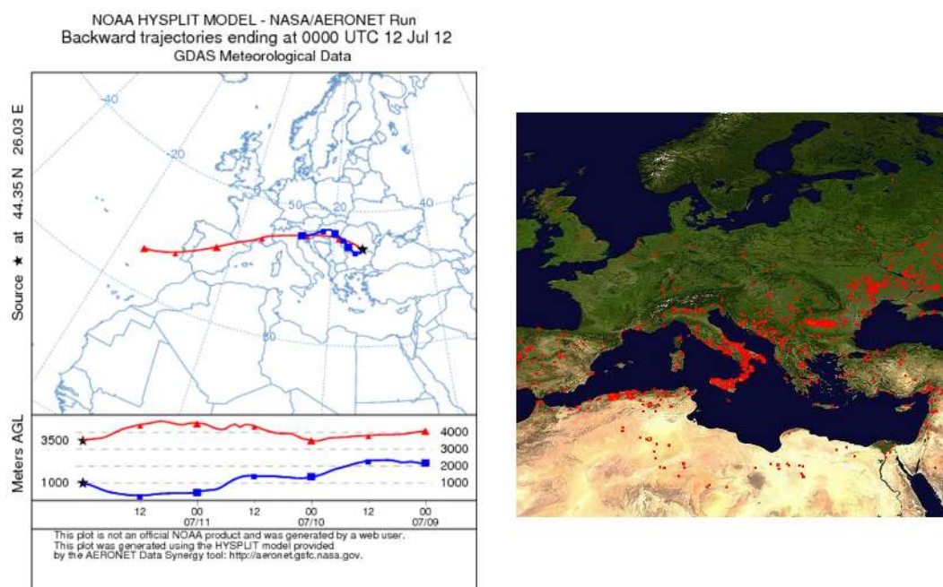
Fig. 8. The result from 72 h back trajectories displaying the air mass arriving on 12 July 2012 at aerosol layer of the altitude 1000 m and 3500 m (blue line and red line each, left panel). Fire areas depicted by MODIS 10 days composite images between 9 and 18 July 2012 (right panel).
