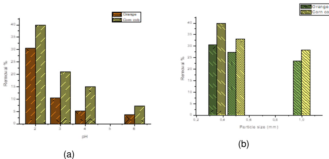
Fig. 3. Effect of (a) pH and (b) particle size in the removal percentage of Cr(VI).
