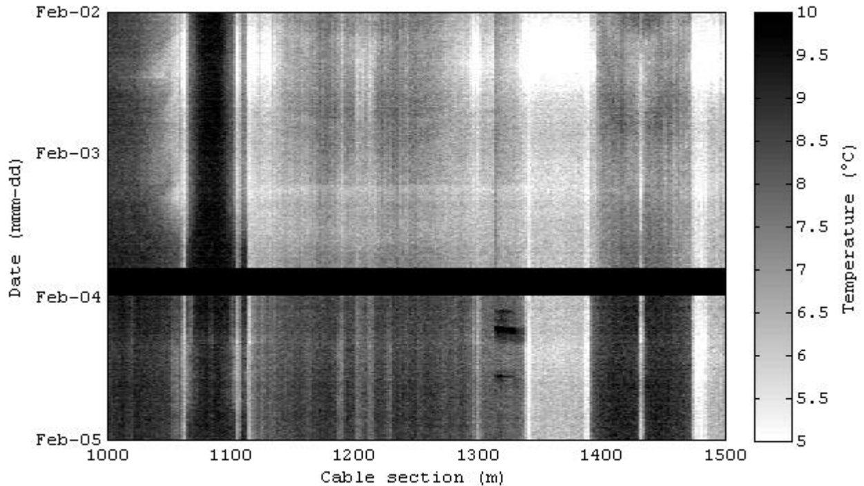
Figure 1: Results from a DTS project in Breda (feb 2012). Until feb 03, the storm sewer was completely filled. From feb 04 the system was kept empty. During the blacked period, measurements stopped because of extreme weather conditions (Air temperatures < -20^{\circ}\text{C} , which is beyond the operational limit of the monitoring equipment). At X=1310 , a clear intermittent discharge, resembling an illicit connection can be noted after feb 04.
