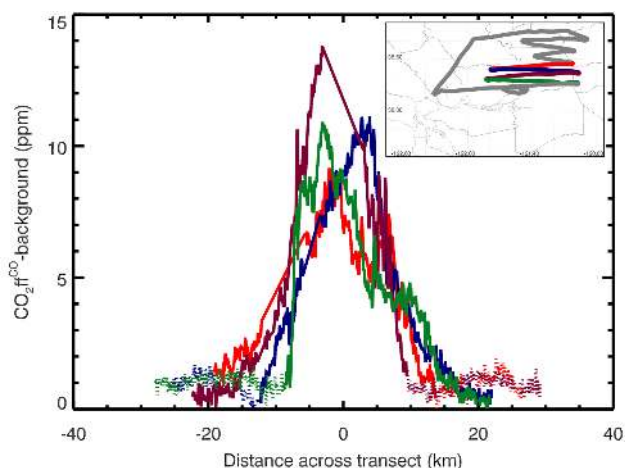
Fig. 9. X_{\text{meas}} ( \text{CO}_2\text{ff}^{\text{CO}} – background \text{CO}_2 ) used to integrate for the flux calculation for each of four downwind transects in SAC227. Solid lines indicate the areas inside the plume for each transect. Inset, flight map showing the individual transects, with the same color coding.
