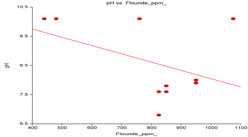
Fig. 1. Correlation and regression plots of pH and fluoride values of toothpastes
