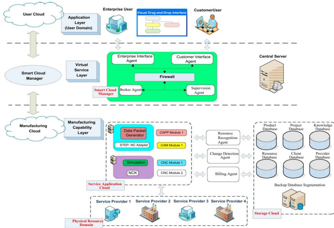
Figure 2: ICMS architecture [25]
