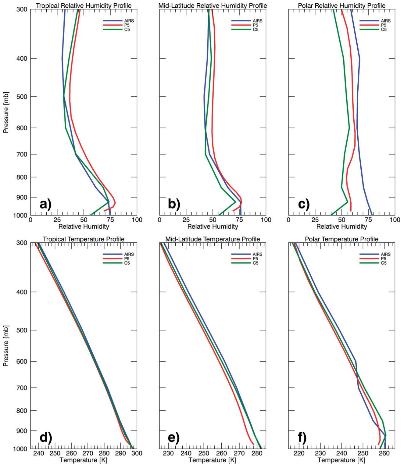
FIG. 8. Vertical distributions of (top) RH and (bottom) temperature from AIRS and NASA GISS P5 and C5 simulations over (a),(d) tropical (30°S–30°N), (b),(e) midlatitude (30°–60° lat both hemispheres), and (c),(f) polar regions (60°–90° lat both hemispheres).
