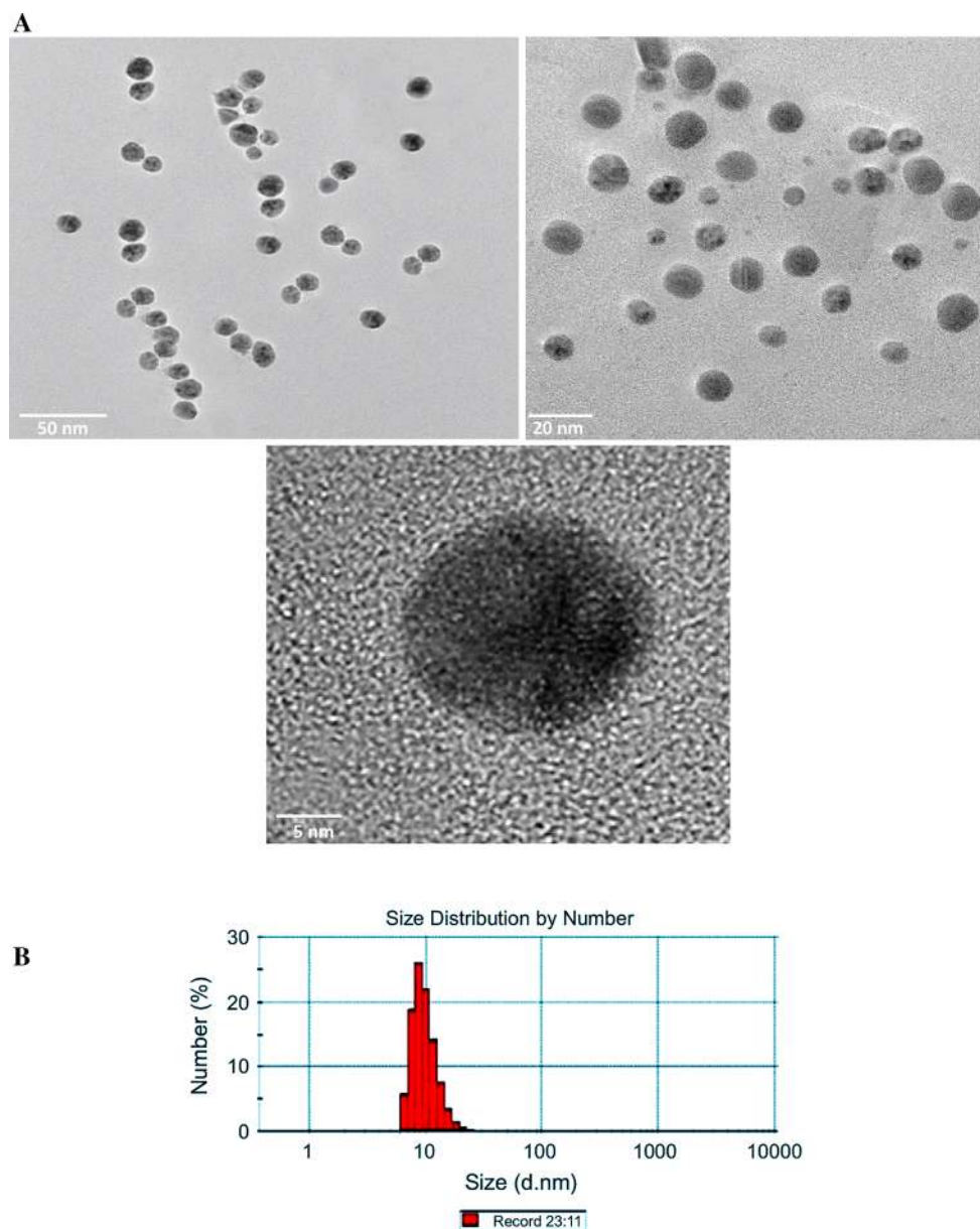
Fig. 2 a HR-TEM images of the mycosynthesized AgNPs at different scales (50, 20 and 5 nm), as indicated. b Particle size distribution analysis
