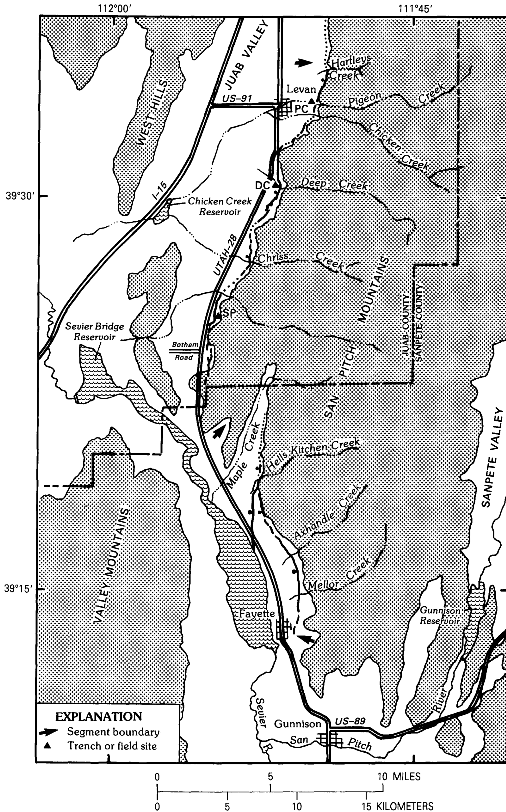
FIGURE 19.—Levan (northern) and Fayette (southern) segments of the Wasatch fault zone. Faults are shown by heavy lines having a bar and ball on the down-dropped side (dotted where uncertain). Also shown are important geographic features and towns. Trench and field sites are abbreviated as follows: PC, Pigeon Creek; DC, Deep Creek; SP, Skinner Peaks.
