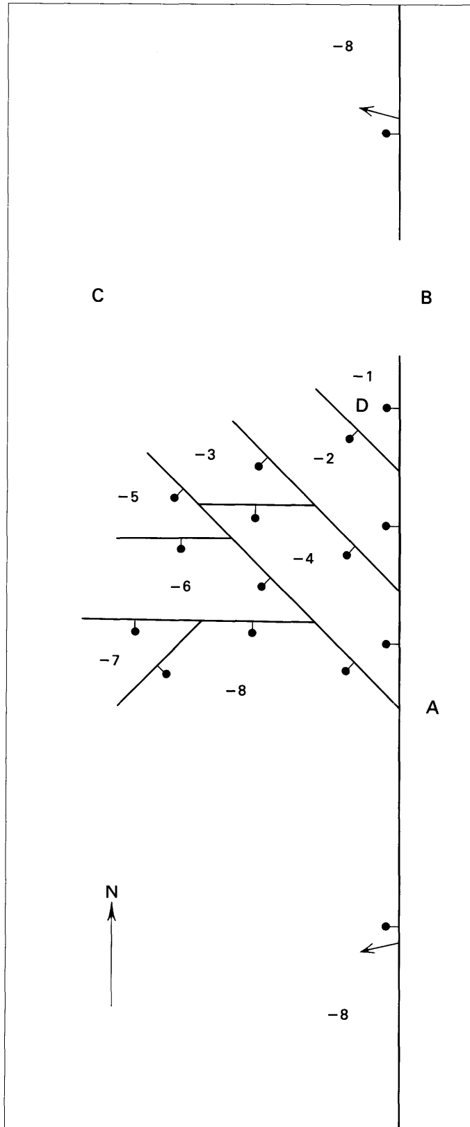
◀ FIGURE 16.—Fault network (process zone) in a hypothetical nonconservative barrier on a normal fault. Solid lines represent traces of faults; bar and ball are on the downthrown side of each fault. Arrows show trends of slip vectors. Numbers give structural elevations (in arbitrary units) with respect to zero elevation of the eastern wall of the main (north-striking) fault strand. A identifies a fork in the fault trace; B and C, two ends of a bedrock ridge; D, a small fault block (all are discussed in the text).
