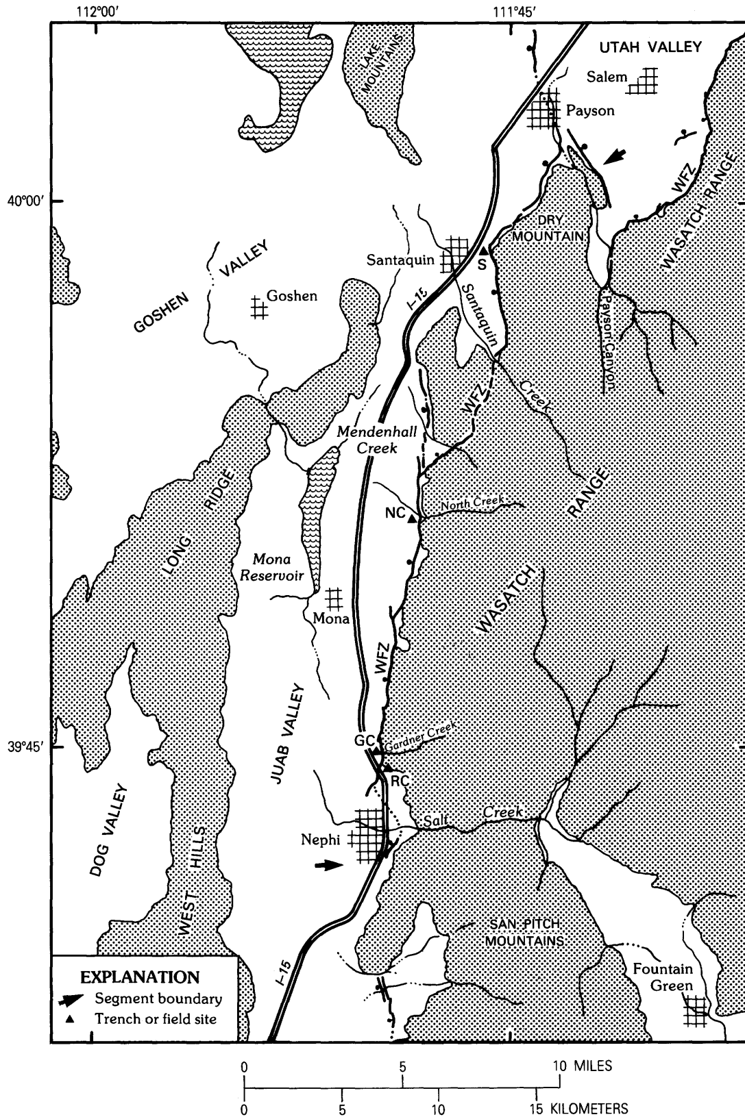
FIGURE 18.—Nephi segment of the Wasatch fault zone (WFZ), which extends from just north of Payson to Nephi, Utah. Faults are shown by heavy lines having a bar and ball on the down-dropped side. The area south of the segment boundary lacks evidence of Holocene faulting. Also shown are important geographic features and towns. Trench and field sites are abbreviated as follows: S, Santaquin; NC, North Creek; GC, Gardner Creek; RC, Red Canyon.
