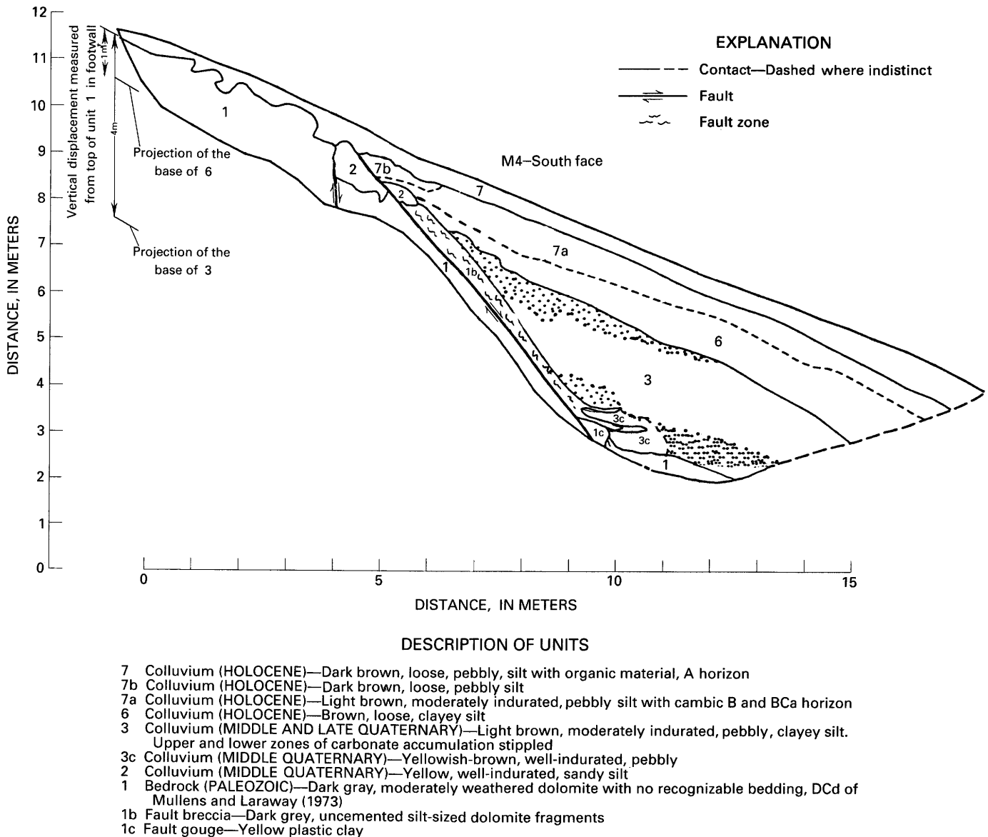
FIGURE 6.—Log of trench M4 at the Robeson Springs trench site, showing faulted middle and late Quaternary colluvial deposits at the southern end of the central section of the Morgan fault. Sloping lines at the left are projections of displaced surfaces (the amount of the displacement is indicated).
