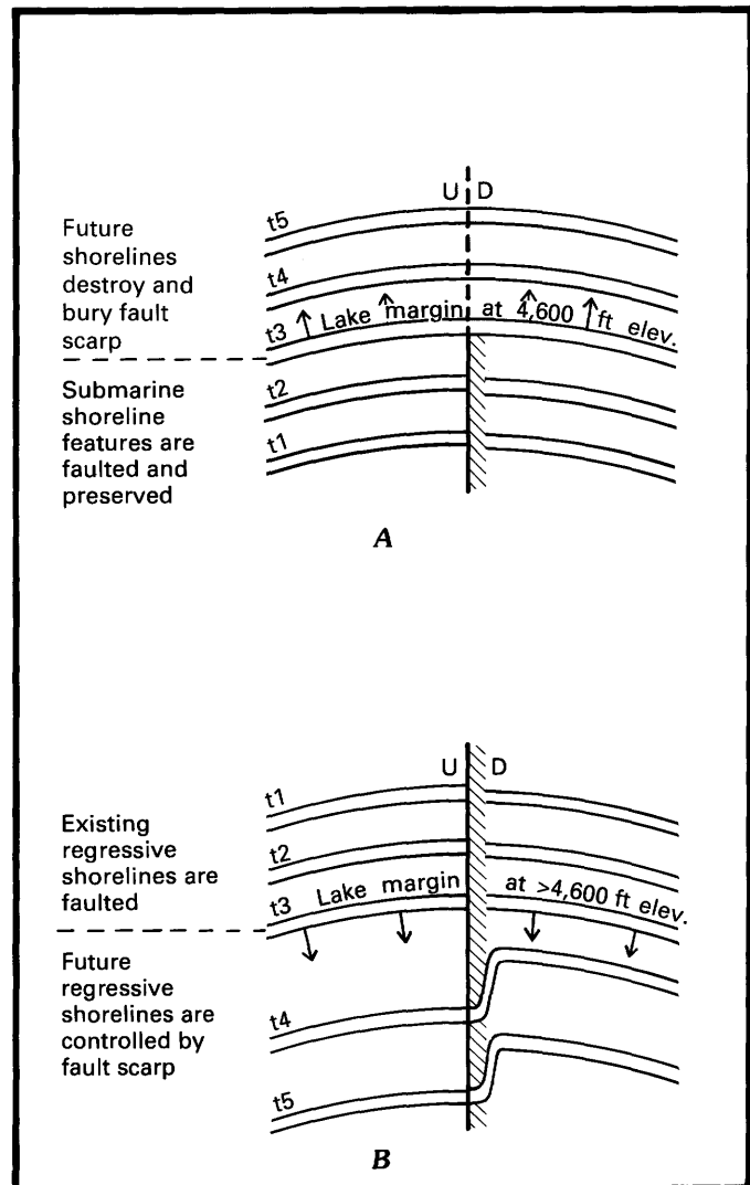
FIGURE 14.—Geomorphic setting of a fault scarp formed during a lacustrine transgression ( A ) and regression ( B ). Time of shoreline occupation is shown by t and progresses from t 1 to t 5. In both instances, hypothetical faulting occurs when the shoreline is at t 3.
