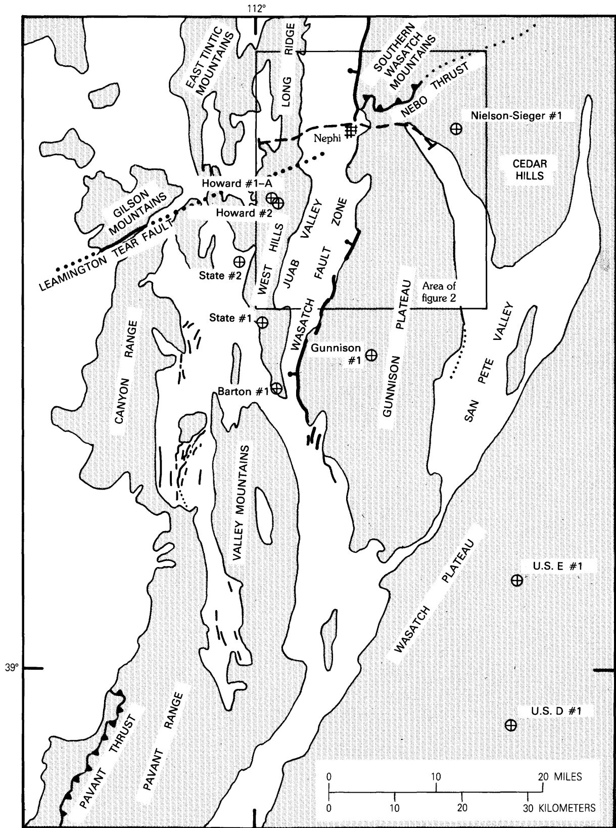
FIGURE 1. — Late Cenozoic normal faults (heavy lines, bar and ball on downthrown side) and Sevier frontal thrust faults (barbed) in central Utah. Ranges are shaded. The Leamington tear fault is shown as a heavy solid line (inferred buried extension shown as a dotted line). Locations of petroleum exploration wells are also indicated. Box shows location of figure 2.
