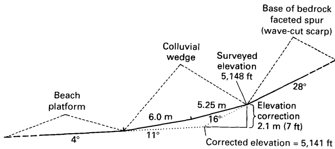
FIGURE 8.—Method used in estimating actual elevations of pluvial lake shorelines covered by Holocene colluvium. The beach platform and wave-cut scarp components are projected beneath the colluvial wedge. The resulting intersection is presumed to be a more accurate representation of the actual shoreline angle.
