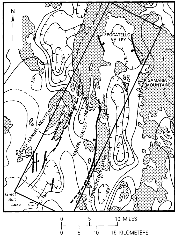
FIGURE 3.— Bouguer gravity anomalies of the Hansel Valley-Pocatello Valley corridor (rectangle) and adjacent areas (from Peterson, 1974). Gravity values are in milligals; contour interval 5 mGal. Stippling represents mountain blocks; heavy lines represent Quaternary faults (dashed where inferred, bar and ball on downthrown side). The gravity low of Pocatello Valley seems to continue southward to Blue Creek Valley rather than southwestward to Hansel Valley.
