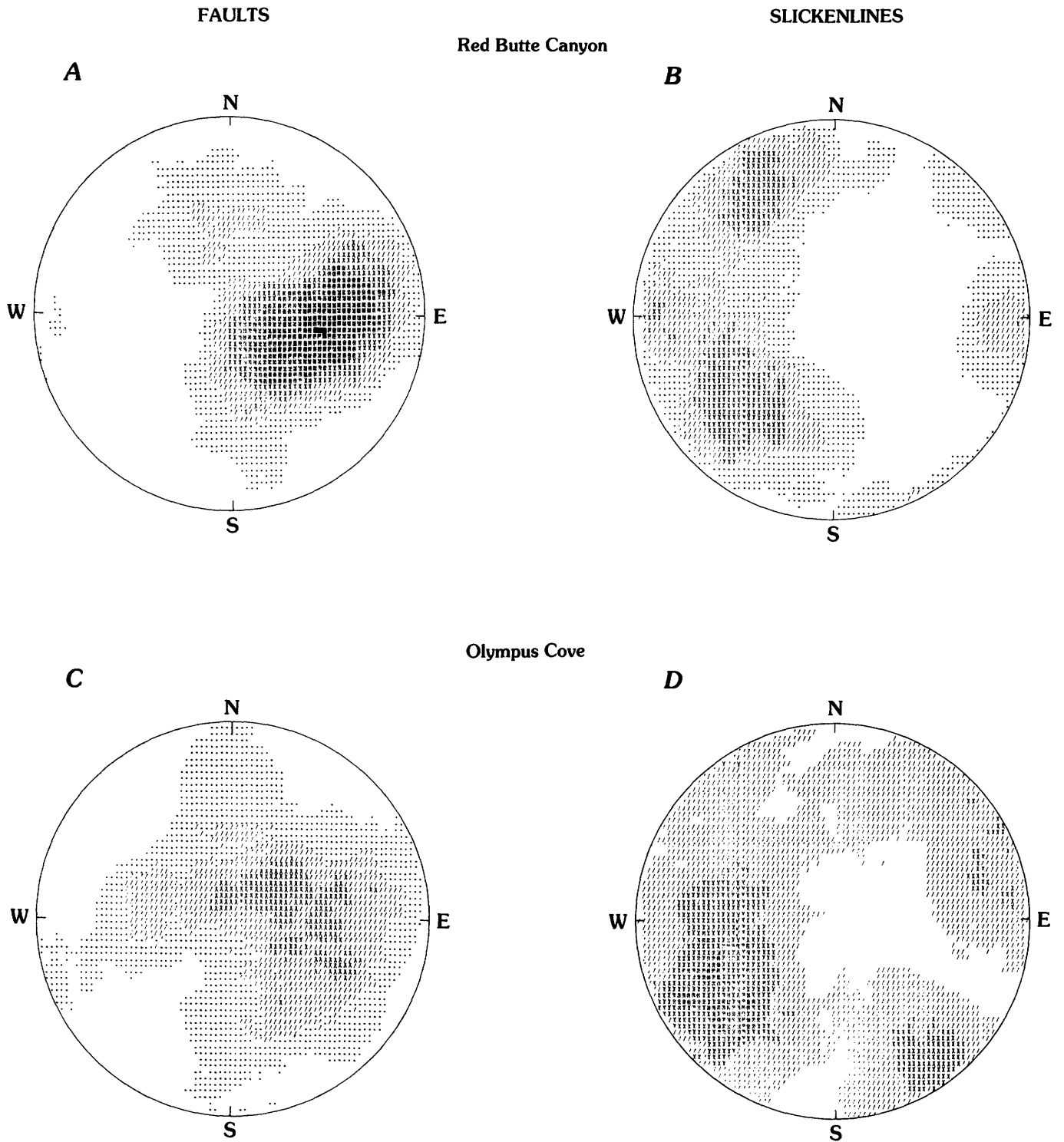
FIGURE 3.—Contoured orientations of poles to fault planes and slickenlines for fault populations in each structural domain in figure 1. Red Butte, 129 measurements of faults (A) and slickenlines (B); Olympus Cove, 105 measurements of faults (C) and slickenlines (D); Draper, 110 measurements of faults (E) and slickenlines (F); Fort
