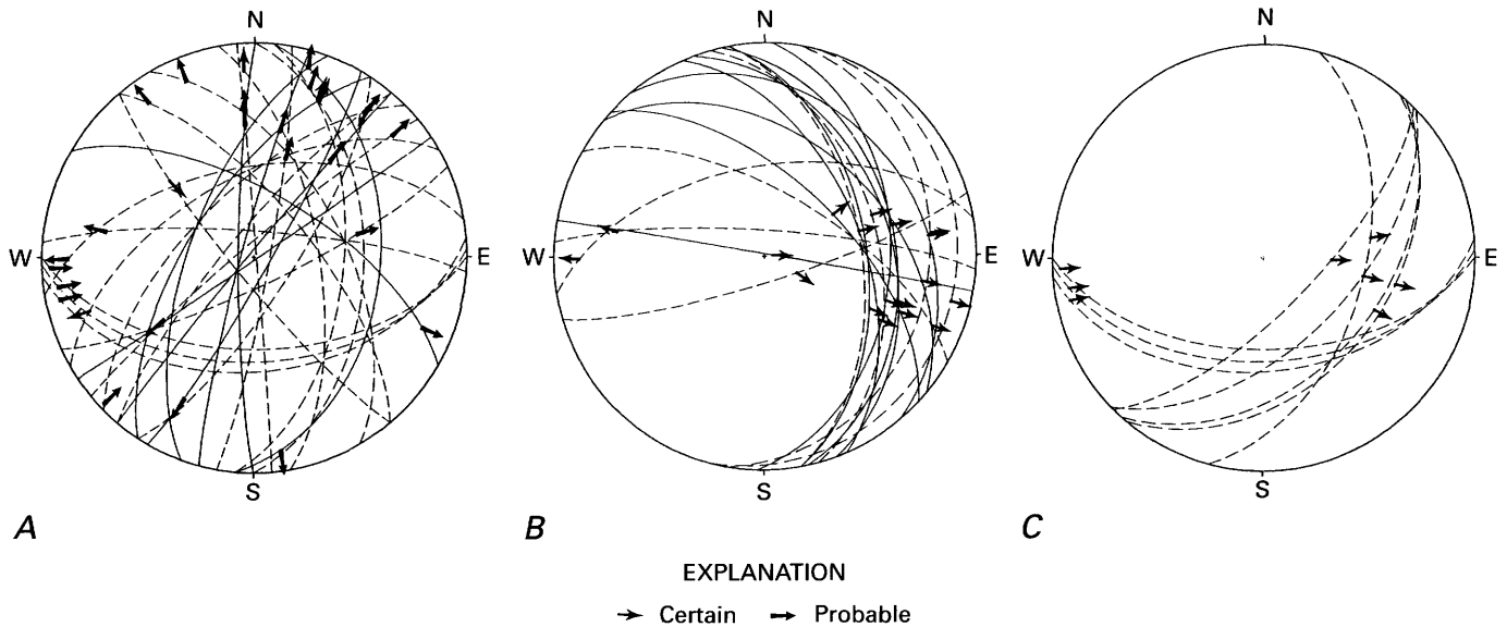
FIGURE 27.—Stereographic plots of faults that cut Tertiary rocks at or above the contact with the mechanically weak Arapien Formation along the southern part of the Sanpete-Sevier anticline. Solid lines are dextral faults; dashed lines are sinistral faults. A, Subsample of 29 predominantly strike-slip faults derived from the sample shown in figure 26A. B, Faults and striae from a group of closely spaced exposures of highly fractured welded ash-flow tuffs on the eastern flank of the anticline. The bases of arrow shafts mark lineations, and
