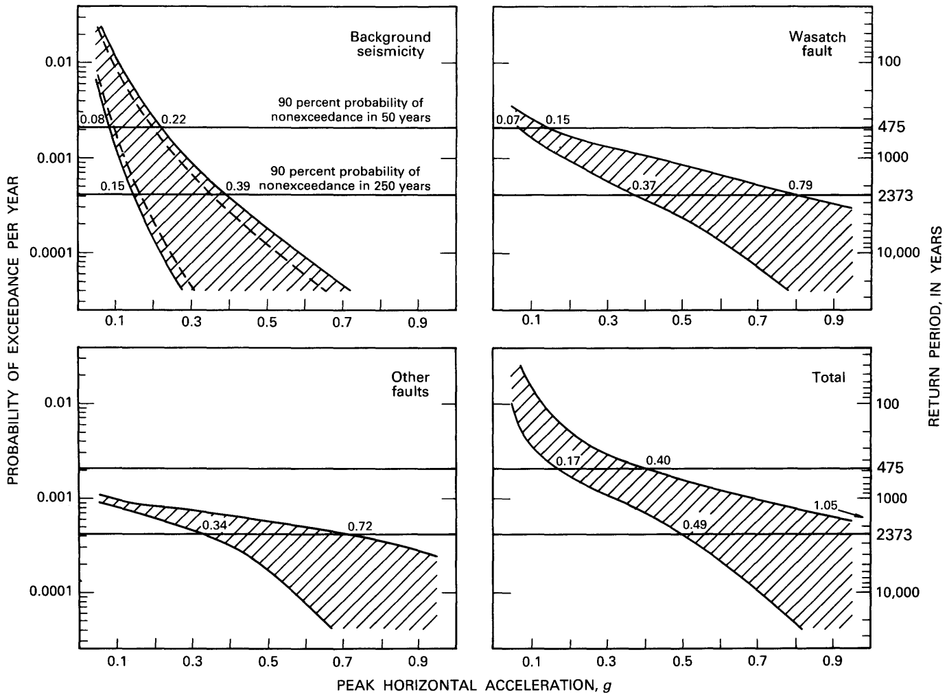
FIGURE 14.—Probability of exceedance per year for peak horizontal ground accelerations on soil at the intersection of I-15 and I-80 in South Salt Lake at approximately 40^{\circ}43.1' N. , 111^{\circ}54.2' W. (diamond, fig. 5). The hachured zones represent the range of values calculated by using the range of median attenuation curves for peak horizontal acceleration presented by Campbell (in press). The results of separate calculations for the background seismicity, the Wasatch fault, other faults (the West Valley, East Great Salt Lake, and North Oquirrh Mountains faults), and all of these sources together are
