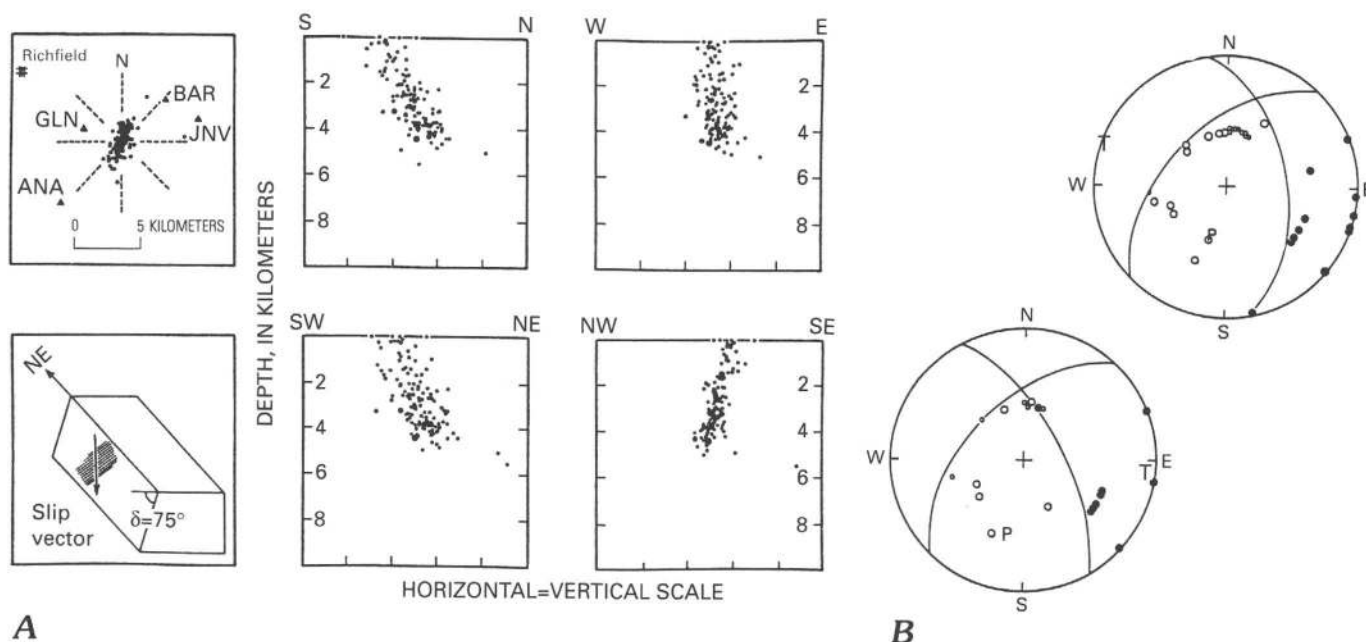
FIGURE 33.—A, Spatial distributions of aftershock foci in the Annabella area (lettered triangles represent seismograph stations). B, Focal mechanisms for the 1982 magnitude 4.0 main shock (upper stereogram) and magnitude 2.7 aftershock (lower stereogram) (from Julander, 1983). The earthquake foci are shown in map view (upper left-hand square) and cross section (center and right-hand squares).
