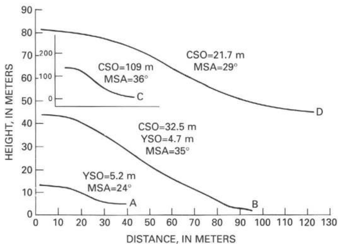
FIGURE 32.—Profiles across scarps formed on late Quaternary alluvium and debris flows in the Annabella area. Profiles A, B, and C cross the main strand of the Sevier fault at localities identified by corresponding letters in figure 31. CSO, cumulative surface offset; YSO, young surface offset; MSA, maximum slope angle. Profiles A and B were measured with a clinometer. At profile A, the fault offsets the youngest terrace above the modern stream bed at the mouth of Water Creek Canyon, whereas the same fault at profile B offsets an older and higher terrace a short distance to the south of A. The young surface-faulting event represented by profile A produced a surface offset of 5.2 m. That surface-faulting event, which probably occurred close in time to the Pleistocene-Holocene boundary, is shown in profile B by a 20-m-long scarp midsegment displaying an average slope near the angle of repose at 35^\circ . This oversteepened part of the compound scarp yields a young surface offset of about 4.7 m, similar to that of the single-event scarp at A. This young faulting event is probably also expressed in the high compound scarp at locality C (note the tenfold scale difference), but it cannot be discriminated, because that profile was constructed from data on the 1:24,000-scale topographic map (Water Creek Canyon, Utah) and therefore only approximates the true surface profile. A remarkably large planar part of the scarp at C stands approximately at the angle of repose (compare profile C with the photograph in fig. 31), indicating numerous late Quaternary faulting events. With a surface offset of about 130 m, it is probably the highest late Quaternary fault scarp in alluvial deposits in Utah. Profile D was measured with a clinometer on a northeast-striking fault scarp 1.5 km northwest of the scarp at locality C. It is included to show that other scarps in the Annabella area do not reflect the same high rates of activity that are found on the main strand of the Sevier fault.
