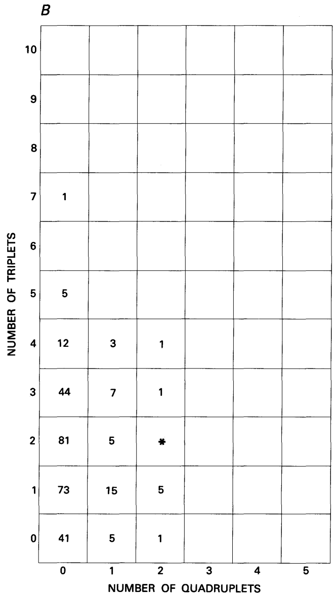
simulated patterns have 1 triplet but no quadruplets; of these patterns, 25 lack quintuplets and plot in the plane of the page, 2 have 1 quintuplet each and plot 1 unit above the page, and 1 has 2 quintuplets and plots 2 units above the page. A , Measured anomaly widths. 300 simulations. B , Minimum widths that are allowed by locational uncertainties of anomaly edges. 300 simulations. C , Maximum allowable widths. 100 simulations. Circled entry at (1, 2) indicates that one of these two simulated patterns also has a sextuplet.
