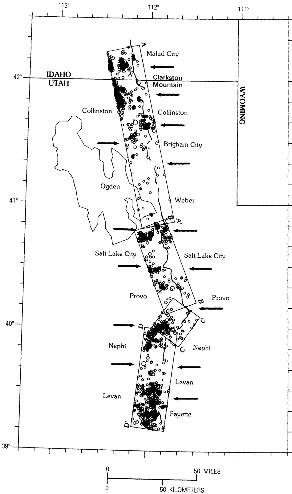
FIGURE 15.—Wasatch fault, segment boundaries and names [according to Machette and others (this volume), right-hand side; Schwartz and Copper-smith (1984), left-hand side], and all earthquakes located by the University of Utah Seismograph Stations during the period July 1962 through December 1986. Circle sizes indicate the relative magnitudes of events.
