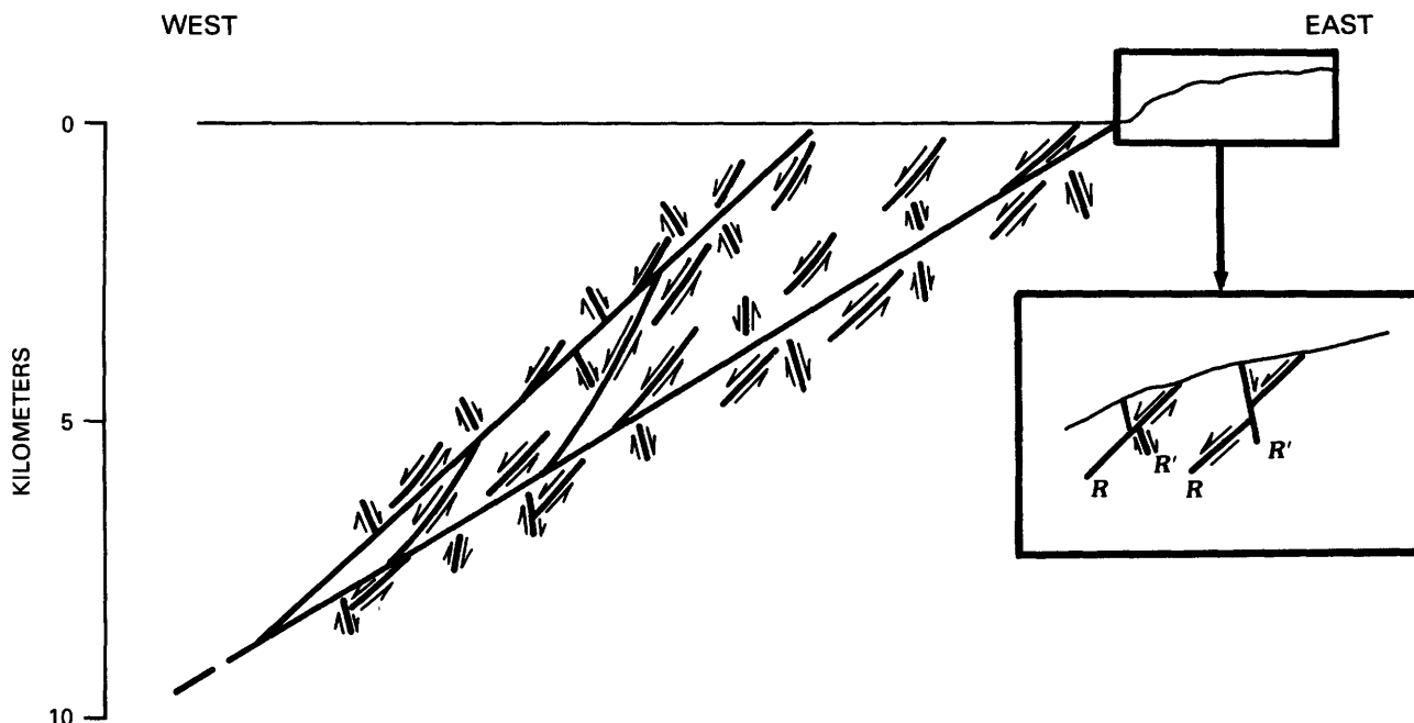
FIGURE 12.—Possible structure of the branched fault zone in the northern half of the Salt Lake segment. Conjugate faults like those in figure 11 are interpreted to pervade the region between the eastern and western primary fault planes. A, The two
