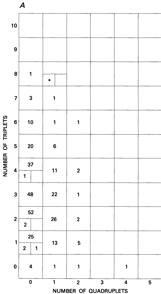
FIGURE 12.—Comparison of numbers of m -tuplets in observed and simulated patterns. Asterisks represent observed patterns. Numerical entries are the numbers of simulated patterns that have the indicated numbers of triplets and quadruplets. Cells that are divided into three subcells record patterns having quintuplets. Upper, lower left-hand, and lower right-hand subcells give the numbers of patterns having zero, one, and two quintuplets, respectively. Zero-valued entries are omitted for clarity. Numbers of quintuplets are plotted along a third axis that rises perpendicularly out of the page. For example, in figure 12A, 28
