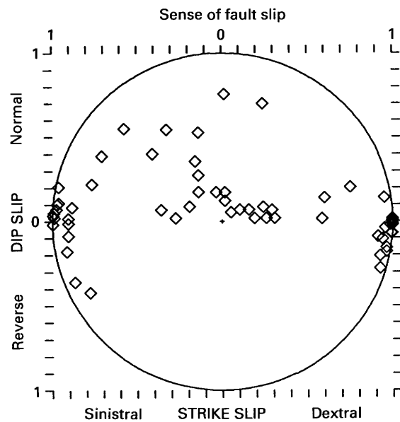
▶ FIGURE 21.—Histograms of strike, dip, and rake, lower hemisphere stereographic plots of computed paleostress axes, and plot of dip-slip versus strike-slip components of fault slip for faults in the western margin of the Sevier Plateau in the Monroe area. The patterned sector on the strike plot is the average range-front trend, 005°±15°. R , radius of the histogram, in number of measurements; N , sample size; D , azimuthal range of dextral faults (number of faults in parentheses); S , azimuthal range of sinistral faults (number of faults in parentheses); d , number of striae that form an angle greater than 45° with the theoretical maximum shear stress; \Delta , mean angular difference between the actual striae and the theoretical maximum shear stress on the fault plane; \Phi = (\sigma_2 - \sigma_3) / (\sigma_3 - \sigma_1) ; \sigma_1 , \sigma_2 , and \sigma_3 , maximum, intermediate, and minimum principal compressional stresses, respectively. The coordinates in the slip-sense plot are the same as those in figure 15.
