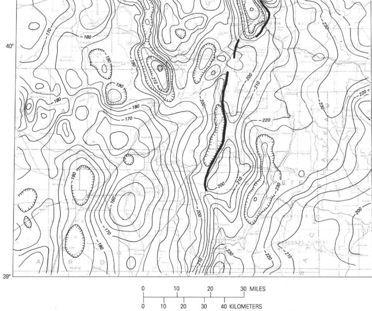
FIGURE 1.—Complete Bouguer gravity anomalies of the Wasatch Front area and the surface traces of the Wasatch and East Cache fault zones. Contour interval is 5 mGal. Gravity map is modified from Zoback (1983).
