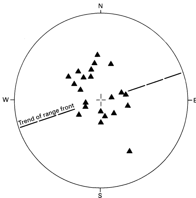
FIGURE 22.—Lower hemisphere plot of poles to bedding in bedrock along the Annabella segment of the Sevier fault. Poles that plot in the southeastern sector mostly represent rocks in the monoclinally flexed or fault-dragged beds of the hanging-wall block, where flexing is away from the range trend (dashed line).
