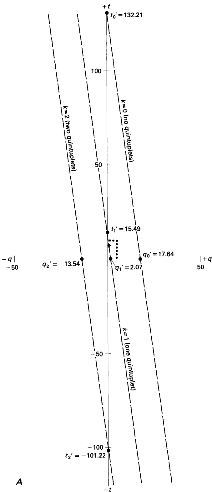
FIGURE 13.—Summaries of serial sections (like the one shown in fig. 4). In notation similar to that of Wheeler and Krystinik (1987a), the number of quadruplets per pattern is q , and the number of triplets is t . Dashed lines are traces of significance plane S' (fig. 4).
