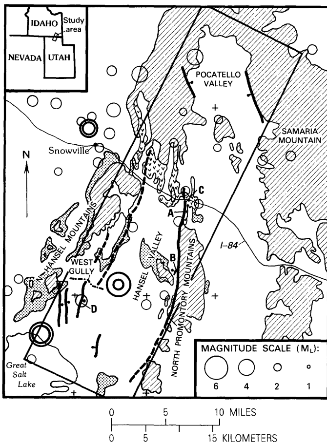
FIGURE 2.— Location and general geology of the Hansel Valley-Pocatello Valley corridor (rectangle). Marginal normal faults discussed in text are shown by heavy lines (dashed where inferred, bar and ball on downthrown side). Earthquake epicenters from 1850 through June 1962 are shown by heavy circles; epicenters from June 1962 through March 27, 1975, are shown by lighter circles. Paleozoic rocks, diagonal pattern; Tertiary volcanic rocks, small v's; Quaternary shoreline gravels, stippling; Quaternary lake-bottom deposits and alluvium, no pattern. A through D locate faults discussed in text.
