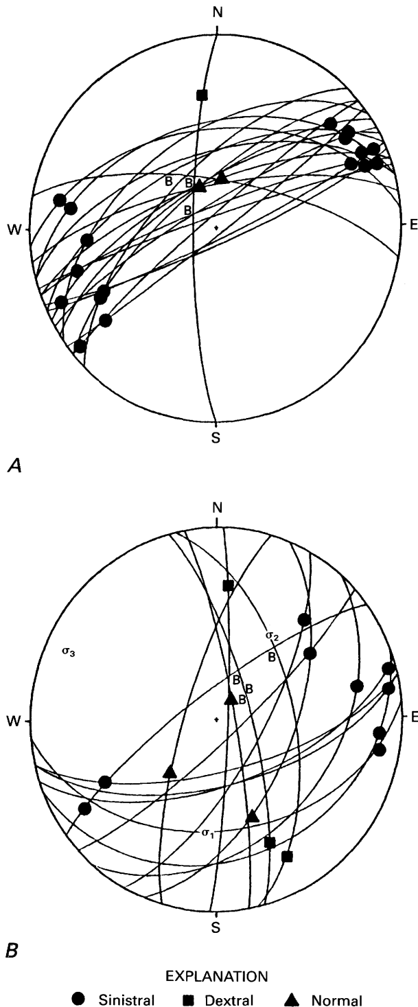
◀ FIGURE 14. — Lower hemisphere plots of fault-slip and bedding data at localities along Interstates 70 and 15. Faults are shown as great-circle arcs, and the striae in those faults are distinguished according to the type of slip. Poles to bedding are shown by the letter B. A, Faults at locality C (fig. 3). Most are sinistral, except for one north-trending dextral fault and two dip-slip faults. The poles to bedding plot near the normal-faulting striae and thus suggest an association between the stratal tilting and the dip-slip components of faulting. B, Faults at locality D (fig. 3). Those that strike between 015^{\circ} and 085^{\circ} are all sinistral or normal sinistral. The remaining are dextral, except for a normal fault exhibiting a steep rake. The faults do not appear to have any simple genetic relationship to stratal tilting. The computed stress axes \sigma_1 , \sigma_2 , and \sigma_3 (maximum, intermediate, and minimum principal compressional stresses, respectively) are poorly constrained because of the small sample size and the predominance of sinistral slip. Nevertheless, the position of \sigma_3 is reasonable in comparison with other computed orientations reported herein (table 1). The moderate inclination of \sigma_1 could result from late-stage rotation of the faults and bedding.
