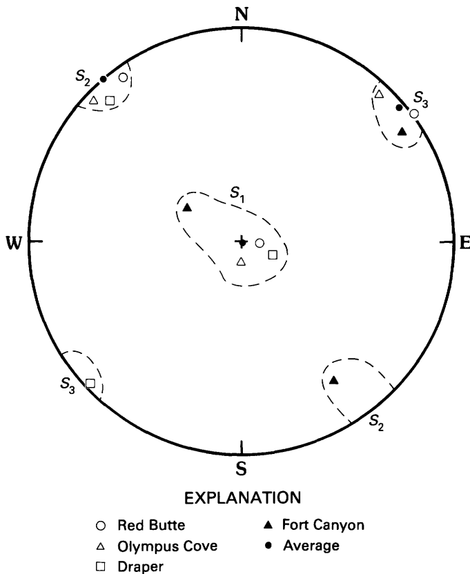
FIGURE 4.—Paleoprincipal deviatoric stress orientations from each of the four structural domains in figure 1 based on inversion of fault-plane and slickenline data. S_1 is the maximum principal compressive stress, S_2 is the intermediate principal stress, and S_3 is the least principal stress. The trend and plunge of each stress axis are shown in table 2.
