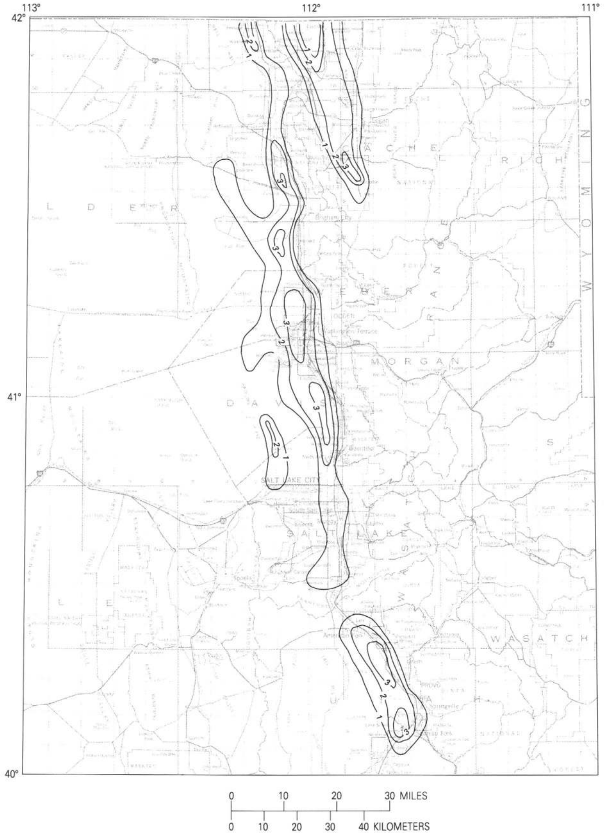
FIGURE 3.—Thickness of low-density sedimentary rocks in Wasatch Front valleys and the Cache Valley, inferred from gravity data. Contour interval is 1 km.
