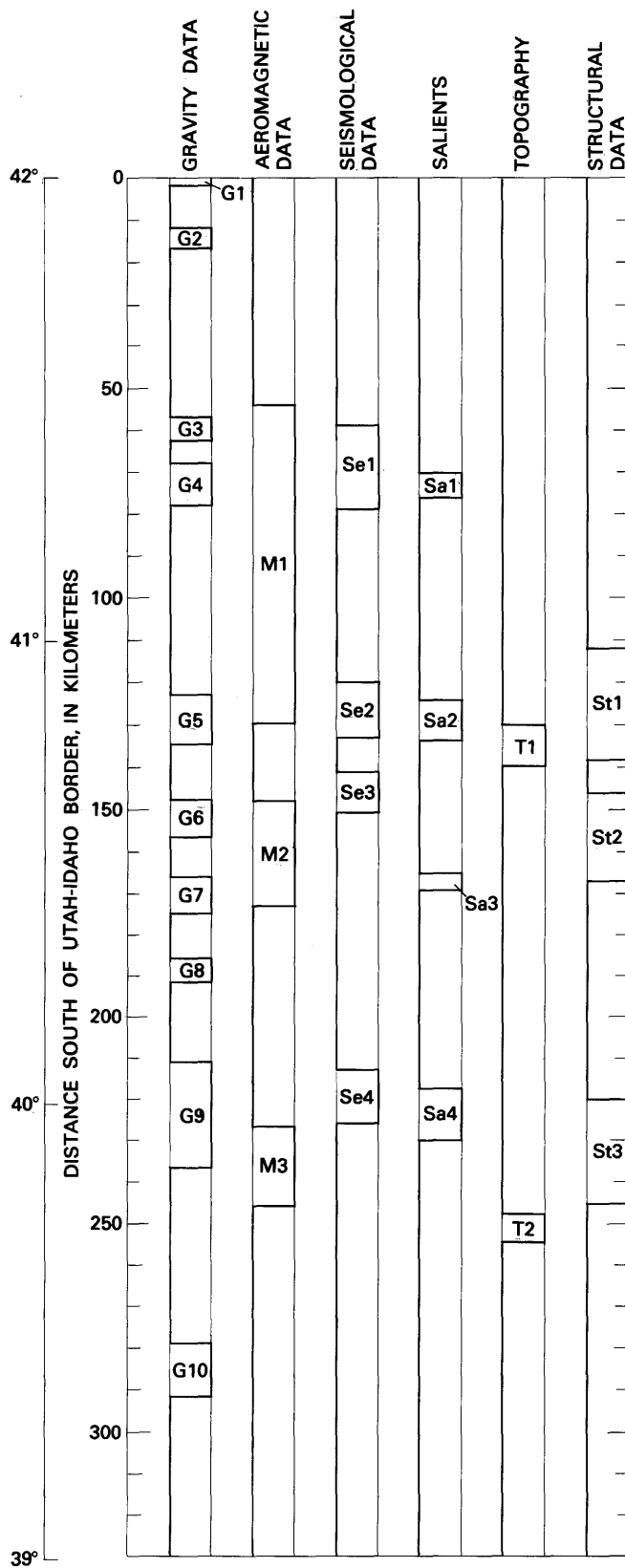
◀ FIGURE 2.—Observed distribution of anomalies along the Wasatch fault zone. The length of the anomaly pattern is 332 km, from the Utah-Idaho border at lat 42° N. to the southern edge of the study area at lat 39° N. Each of the six data types is represented by a vertical line that steps to the right at one end of an anomaly and back to the left at the other end. Anomaly locations and letter-number names are from Wheeler and Krystinik (1988).
