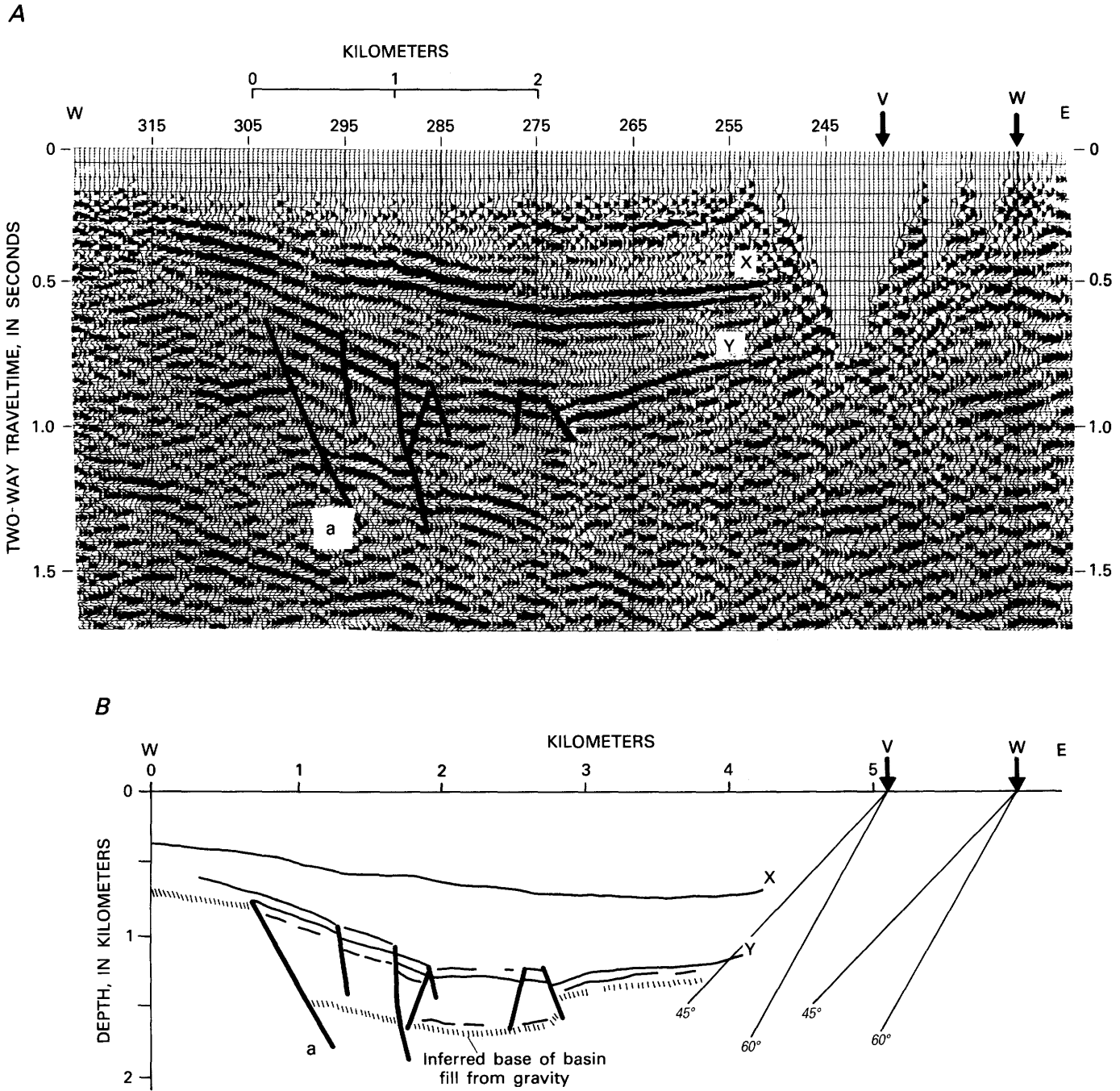
FIGURE 6.—A, Detail of seismic reflection profile in Juab Valley showing basin fill. V and W mark possible surface locations of the Wasatch fault zone described in text. Vibrator points are numbered across the top of the section. A major fault on the western side of the basin is labeled a. Reflectors X and Y are discussed in the text. Heavy
