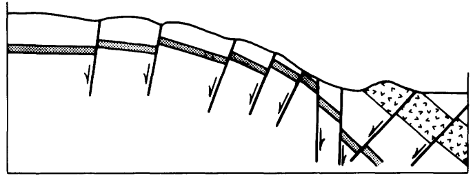
FIGURE 19.—Typical fault offsets seen in the monoclinally flexed margin of the Pavant Range. Fault offsets are similar to those described and analyzed by Thompson and White (1984); patterned beds are hypothetical. Down-to-range faults cut bedding at approximately right angles, and bedding is not rotated by the steep down-to-valley faults.
