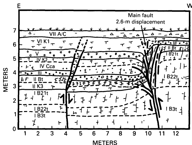
FIGURE 11.—Fault exposed on the southern side of the Rattlesnake Pass (Interstate 84 roadcut (C, fig. 2). Four paleosols are exposed in the eastern two-thirds of the cut, developed on parent materials of unit I (horizons B21t, B22t, and B3t), unit II (horizons Bt and K3), unit IV (horizons K2 and Cca), and unit VII (horizon A/C) plus unit VI (horizon K1). The main fault displaces units I through III by 2.6 m. Units IV and V have evidently been eroded from the upthrown block west of the main fault, and unit VI is considerably thinner on the upthrown block, probably the result of scarp relief. Unit VIII (Holocene? colluvium) is not faulted. Pattern intensity indicates the degree of secondary carbonate or clay enrichment in soil horizons.
