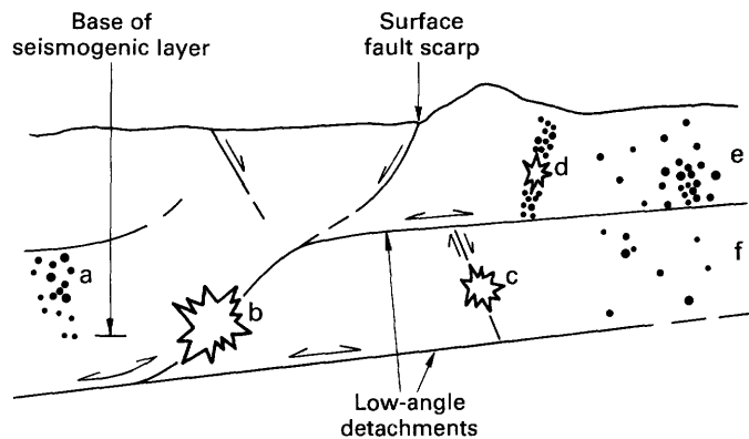
FIGURE 11.—Schematic geologic cross section illustrating the complex association of seismicity in the upper crust with geological structure in the Intermountain Seismic Belt (from Arabasz, 1984; Arabasz and Julander, 1986). Starbursts indicate foci of moderate to large earthquakes; solid circles, microseismicity; lines in subsurface, faults. Arrows indicate sense of slip on faults; two-directional arrows show extensional backsliding on preexisting low-angle faults possibly formed as thrust faults. The base of the seismogenic layer is at a depth of approximately 10 to 15 km. Lowercase letters identify aspects (not exhaustive) of observations and a working hypothesis relating seismicity to structure: a, local predominance of seismicity within a lower plate; b, nucleation of a large normal-faulting earthquake near the base of the seismogenic layer, hypothetically on an old thrust ramp, with linkage or an established rupture pathway to a major surface fault; c, occurrence of a moderate-sized earthquake within a lower plate, without linkage to a shallow structure; d, occurrence of a moderate-sized earthquake and aftershocks on a secondary fault where an underlying detachment restricts deformation to the upper plate; e, diffuse block-interior microseismicity predominating within an upper plate, perhaps responding to extension enhanced by gravitational backsliding on an underlying detachment; f, diffuse block-interior microseismicity within a lower plate where frequency of occurrence is markedly lower than it is in the overlying plate.
