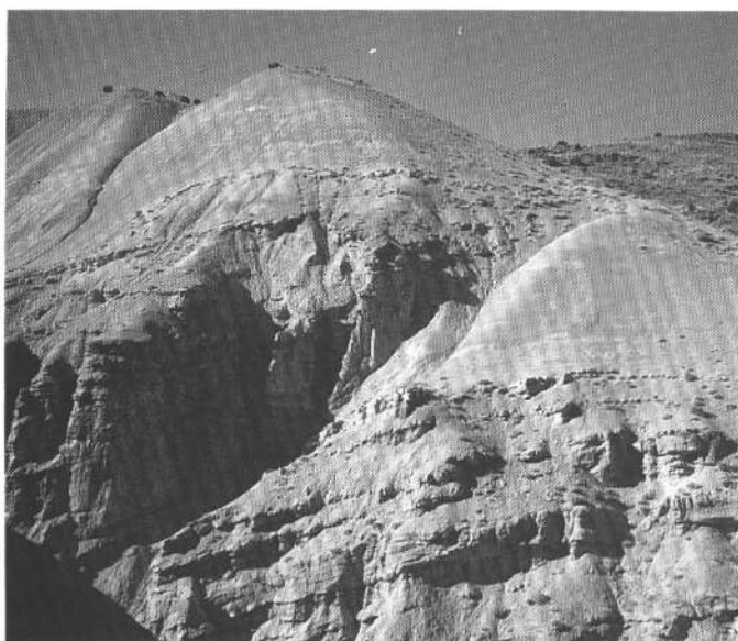
FIGURE 16.—View looking west in Flat Canyon north of Elsinore showing the offset contact between smooth- and rough-weathering beds of gently southwest-dipping sandstone, siltstone, and claystone belonging to the formation of Aurora of late Eocene age (Willis, 1986). The fault that separates the offset sections is approximately vertical, strikes 005°, and has an estimated down-to-the-east throw of 10 m. At first glance, this fault and another nearby fault of similar orientation and displacement but out of camera view appear to be steep dip-slip faults that repeat the strata by down-to-the-east (lower right) displacements. However, as is the case with the faults at locality C (fig. 3) along the Clear Creek downwarp, these faults are sinistral strike-slip faults having rakes of 3° and 13° to the south.
