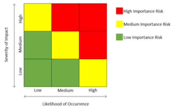
Fig 1: Risk Matrix
