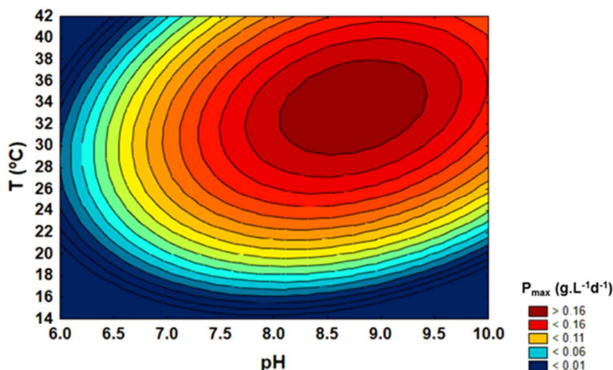
Fig. 2. Contour plot of maximum biomass productivity ( P_{max} ) determined for the set of temperature (T) and pH combinations tested. All growths were carried out at 155 \mu\text{mol photons}\cdot\text{m}^{-2}\cdot\text{s}^{-1} and using a \text{CO}_2 -rich atmosphere (5.5% (v/v)).
