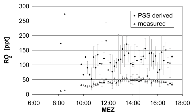
Fig. 9. Mean diurnal variation of measured and PSS derived RO 2 -radicals for the sector 0–80° and the time period of 18.6.–6.7.2000. Error bars refer to the 1 \sigma -standard deviation.
