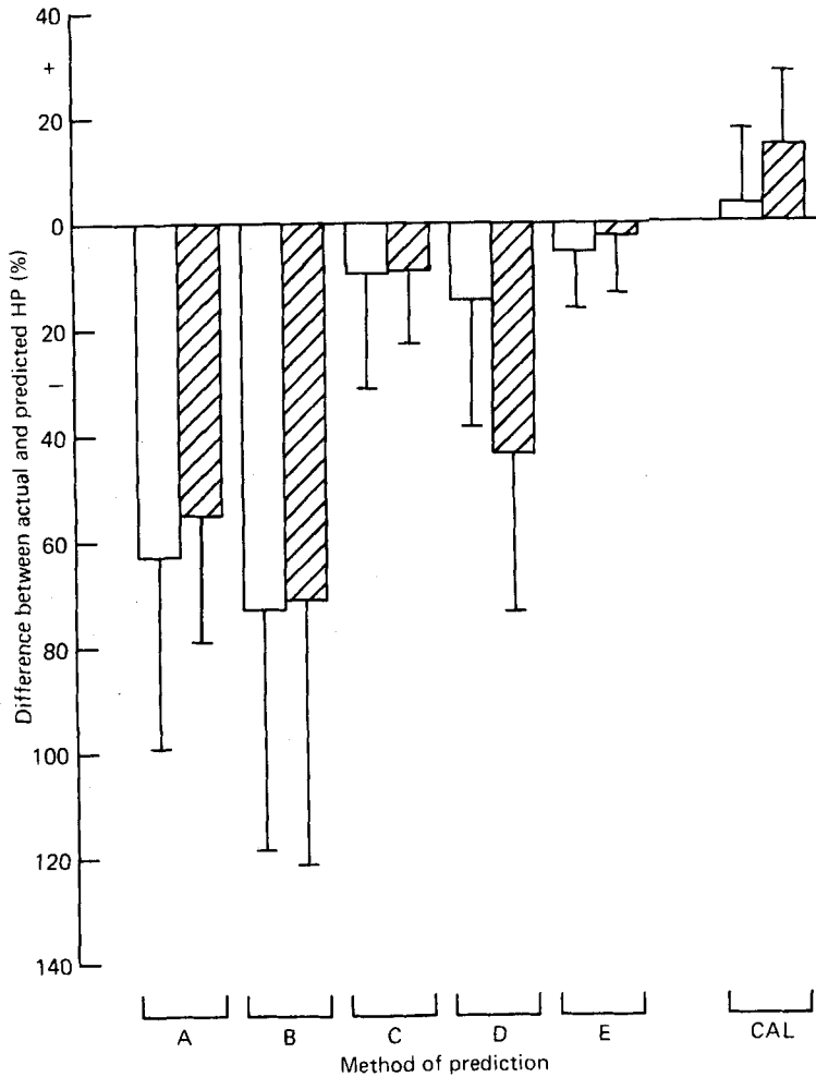
Fig. 5. Percentage differences between actual and predicted values for night-time heat production (HP) (22.30–08.30 hours on days 1–2) obtained using six methods of prediction (see Figs. 1 and 2), for both light (□) and moderate (▨) sessions of activity. The mean values and standard deviations, represented by vertical bars, for the eight subjects are given. CAL, Calorimeter method: for details of methods A–E and CAL, see pp. 4–6.
