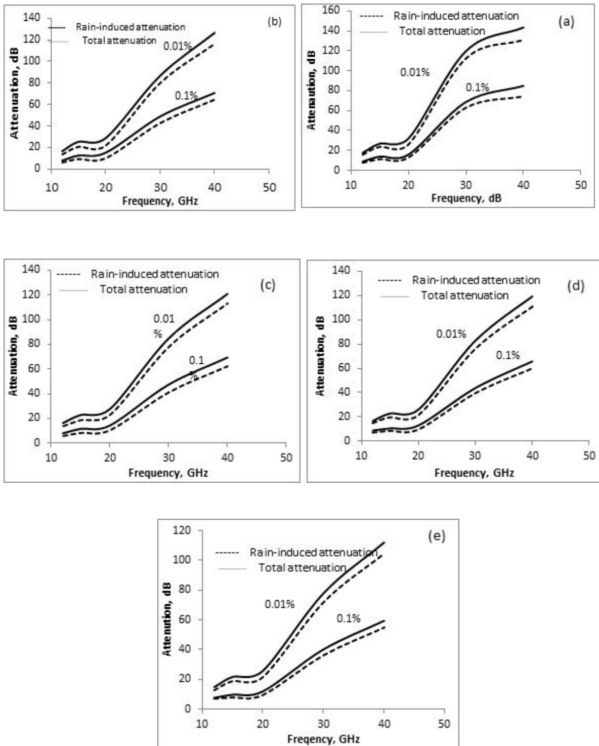
Fig. 7. Comparison of total impairments with rain-induced attenuation at different frequencies time for 0.01 and 0.1% of the time at (a) PH (b) Akure, (c) Ilorin, (d) Zaria and (e) Kano.
