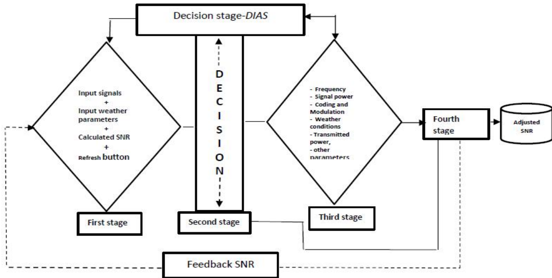
Fig. 2. DAIS algorithm for achieving good QoS.
