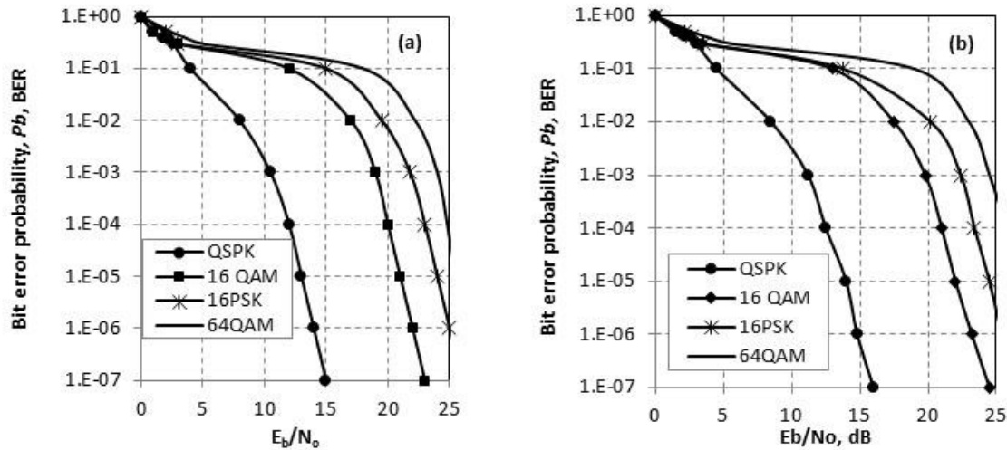
Fig. 9. Typical plots of BER estimated for four modulation schemes at (a) 21.751 GHz and (b) 40 GHz.
