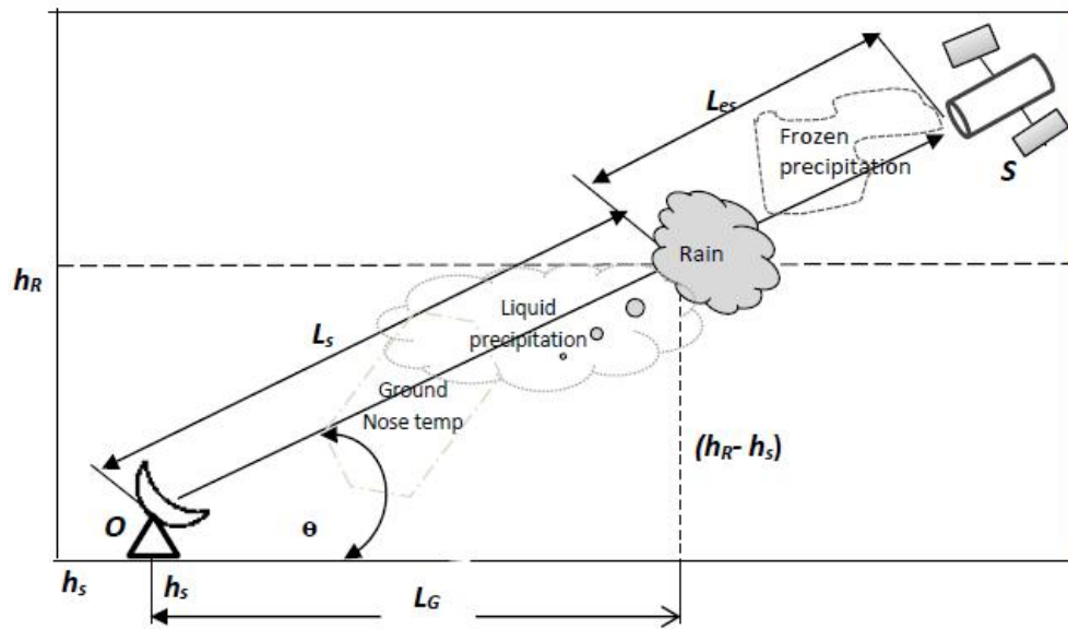
Fig. 1. A typical scenario of total impairments along Earth-space path.
