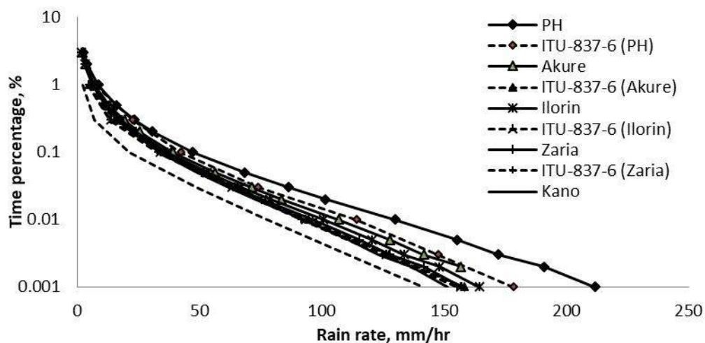
Fig. 4. Comparison of CCDF of measured rain rate with the predictions of ITU-R 837-6 (2012) for all the study locations.
