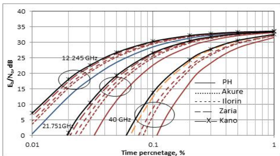
Fig. 8. Variation of CCDF of E_b/N_o slope for a QAM modulation scheme at different frequencies.
