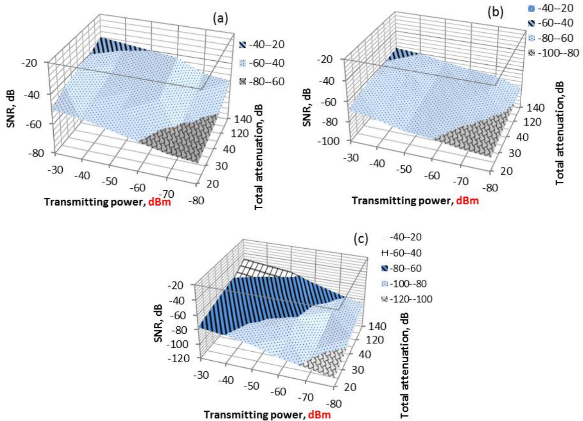
Fig. 11. Typical results of the variation of total impairments and transmitting power on outputs SNR before enhancement for a worst case scenario at (a) 12. 245 (b) 21.751 and (c) 40 GHz frequency.
