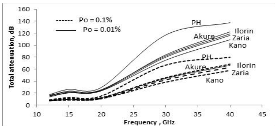
Fig. 6. Influence of total impairments on propagation frequencies for equiprobable exceedance probability 0.01\% < P \leq 0.001\% .
