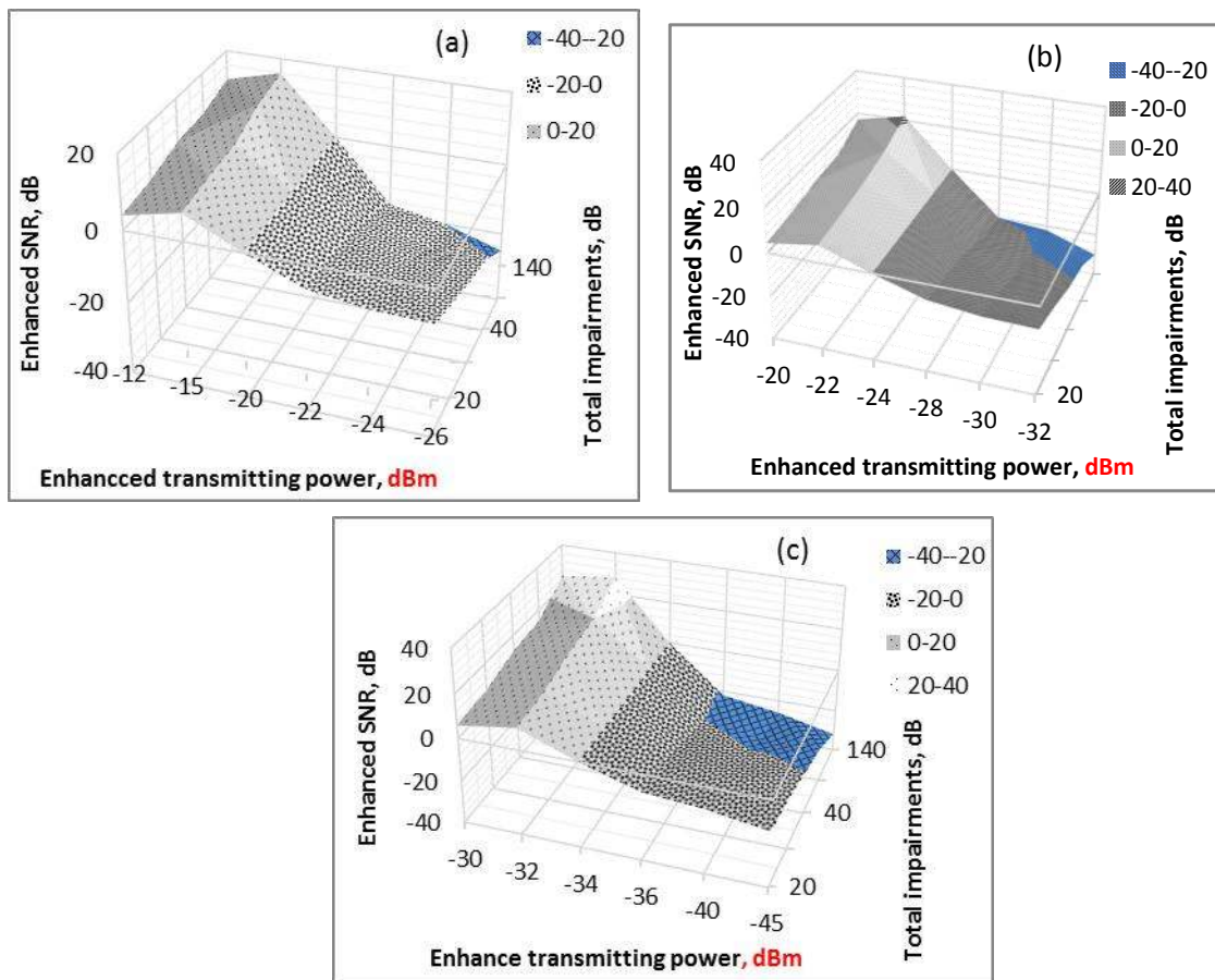
Fig. 12. Typical results of the variation of total impairments and enhanced transmitting power on enhanced SNR for a worst case scenario at (a) 12.245 (b) 21.751 and (c) 40 GHz frequency.
