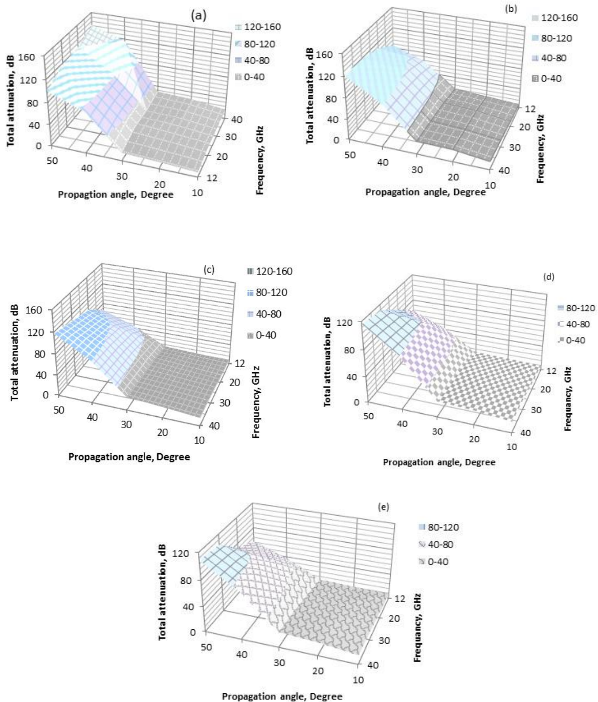
Fig. 10. Variation of total impairments and propagation angles at different satellite propagation frequencies between 12.245 and 40 GHz for (a) PH (b) Akure (c) Ilorin (d) Zaria and (e) Kano.
