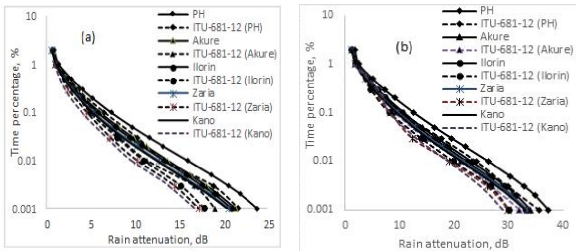
Fig. 5. Comparison of CCDF of measured rain attenuation for (a) 12.245 and (b) 21.751 GHz.
