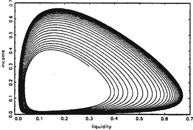
Fig. 4.1. Phase Portrait
