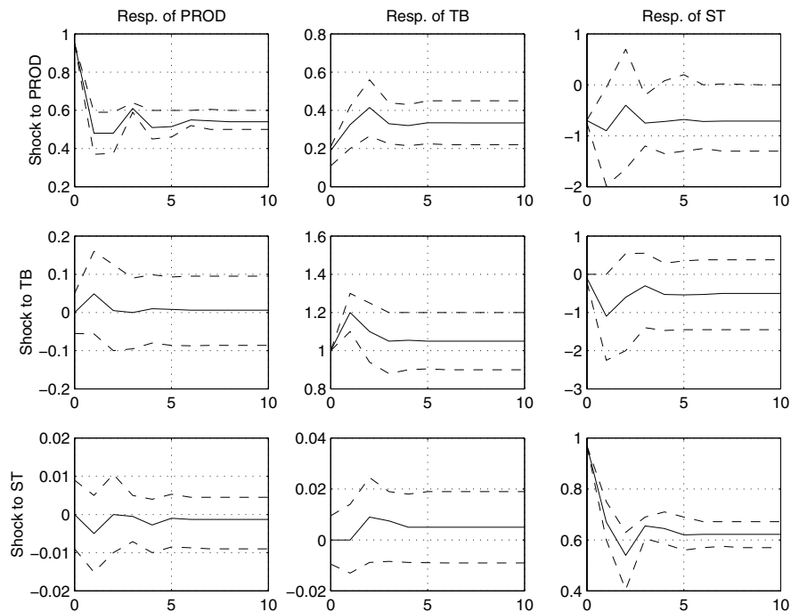
Fig. 5.2. Cumulative Impulse-Responses
