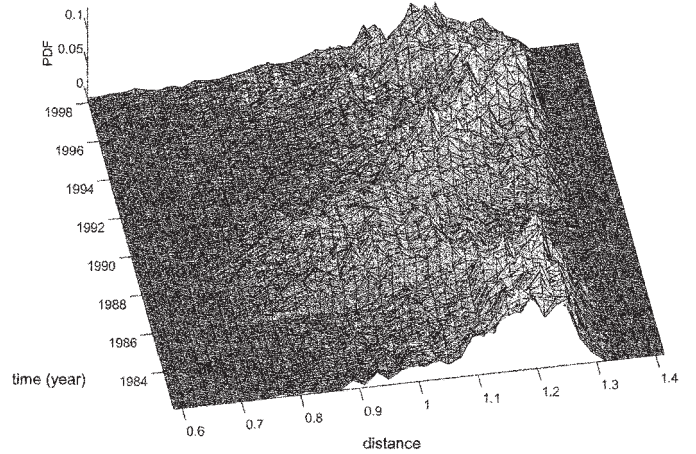
Fig. 4. Distribution of the (N-1) distance elements d_{ij} contained in the asset (minimum spanning) tree T' as a function of time.
