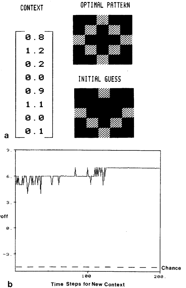
Fig. 8a and b. Example 3. With the associative matrix obtained after training in Example 2, context vector X^1 of Fig. 7a was corrupted by additive noise and presented to the ASN. a The corrupted context vector, the optimal output pattern, and the ASN’s initial guess b ASN payoff as it searches for the optimal output pattern
