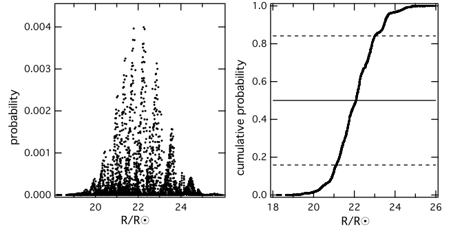
Fig. 7. The projected probability (left) and cumulative probability (right) distribution functions for the radius of the artificial test star 6 (Basu et al. 2010). The full horizontal line correspond to the median and the dashed lines give the \pm 1\sigma confidence interval.
