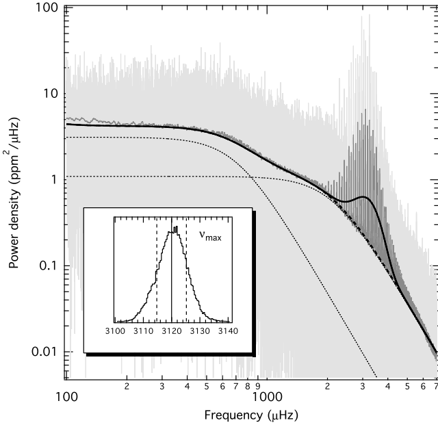
Fig. 5. Power density spectrum of a 1-year VIRGO time series (light-grey) and the corresponding global model fit (black line). The dark-grey line shows a smoothed ( 5 \mu\text{Hz} boxcar filter) version from the average of nine consecutive 1-year VIRGO time series. The inset gives the probability density function for \nu_{\text{max}} with the vertical solid and dashed lines indicating the median value and the 1\sigma limits, respectively.
