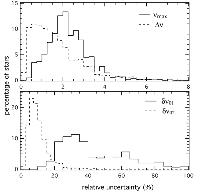
Fig. 4. Histograms of the relative uncertainties for \nu_{\max} , the large frequency separation \Delta\nu , and the small separations \delta\nu_{01} and \delta\nu_{02} .
