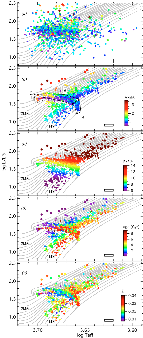
Fig. 9. H-R diagram showing the location of our red-giant sample as directly determined from Eqs. (4) and (5) using the KIC effective temperatures (panel a) and from the comparison with the stellar model grid (panel b) to e)). The colour code (in the online version only) indicates the stellar mass (a) and b)), radius c)), age d)), and metallicity (e)), where the radius scale has been truncated below 6 and above 14 R_{\odot} . Grey lines show solar-metallicity BaSTI evolutionary tracks. The boxes given in the lower right corners illustrate typical uncertainties.
