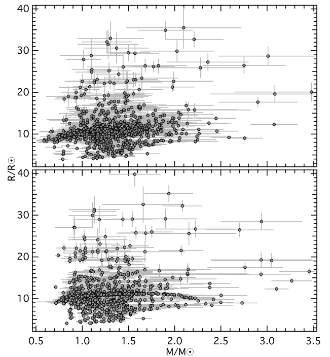
Fig. 8. The stellar radius as a function of mass for the sample of red giants as directly determined from Eqs. (4) and (5) using the KIC effective temperatures (top) and from the comparison with the stellar model grid (bottom).
