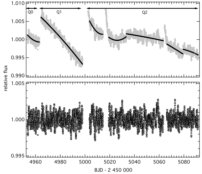
Fig. 1. Relative flux for the Q0, Q1, and Q2 data of KIC 6838420. The top panel shows the original time series (grey points) with the 2nd order polynomial fits overlaid (black lines). The bottom panel shows the residual time series.
