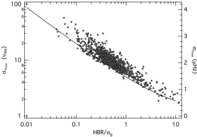
Fig. 3. The uncertainty in \nu_{\max} in actual value (right axis) and in units of the frequency resolution as a function of the ratio between the height-to-background ratio (HBR) and the width of the power excess, \sigma_g . The line indicates a power-law model for the lower envelope.
