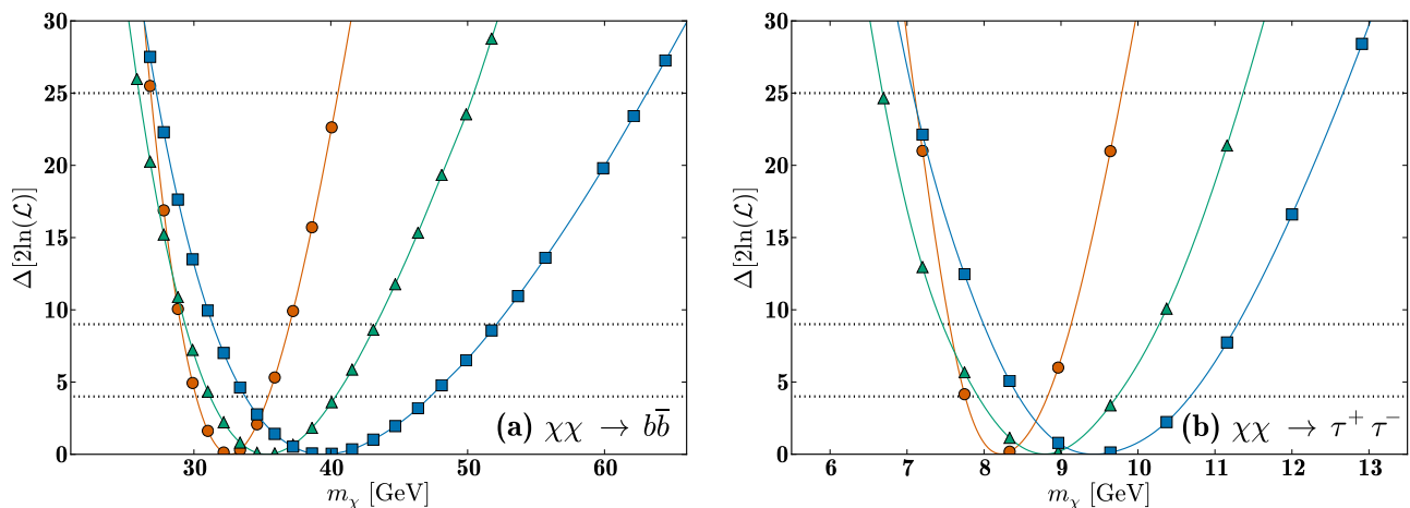
FIG. 9. Shown are the 2\Delta\ln(\mathcal{L}) for the best fit dark matter particle masses for (a) pure b\bar{b} and (b) pure \tau^+\tau^- annihilation channels, for several astrophysical model cases studied when varying all sources on the GC ROI. In both panels, the cases for 2FGL+2PS+GCE show the exact particle mass runs in orange circles, 2FGL+2PS+I+MG+GCE case in green triangles and the full best fit model 2FGL+2PS+I+MG+ND+GCE case in blue squares. Fourth order spline interpolations are shown as lines for each case, which are used to find the minima and limits. For the full 2FGL+2PS+I+MG+ND+GCE model, the b\bar{b} and \tau^+\tau^- are equivalent in their goodness of fit, and there is no evidence for a mixed channel. The horizontal lines are for 2, 3 and 5 \sigma limits.
