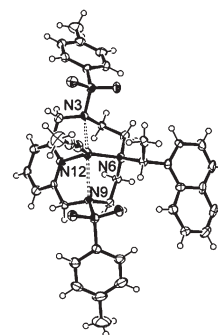
Fig. 7 Structure of compound 10d (thermal ellipsoids are shown at 50% probability level; the [\text{CF}_3\text{SO}_3]^- counter ion is omitted for clarity). Selected bond distances (Å) and angle ( ^\circ ): Cu–N12 2.058(4), Cu–N6 2.111(5), Cu–N3 2.567(4), Cu–N9 2.549(5), Cu–N(CH 3 CN) 1.898(5), N3–Cu–N9 139.1(1). 8 For sake of comparison with 4d , 5d and 6d , N6...N12 is 3.306(5) and N3...N9 is 4.793(6).
