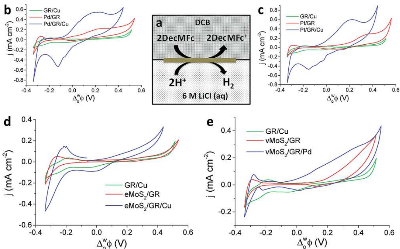
Figure 5. a) Schematic of the HER at the interface. b–e) Cyclic voltammograms at 6 \text{ M LiCl}_{(\text{aq})}/\text{DCB} interface, comparing Pd/GR (b), Pt/GR (c), e\text{MoS}_2/\text{GR} (d), and v\text{MoS}_2/\text{GR} (e) heterostructures assembled at the interface, using a scan rate of 50 \text{ mV s}^{-1} .
