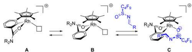
Scheme 2. Stereochemical Model
