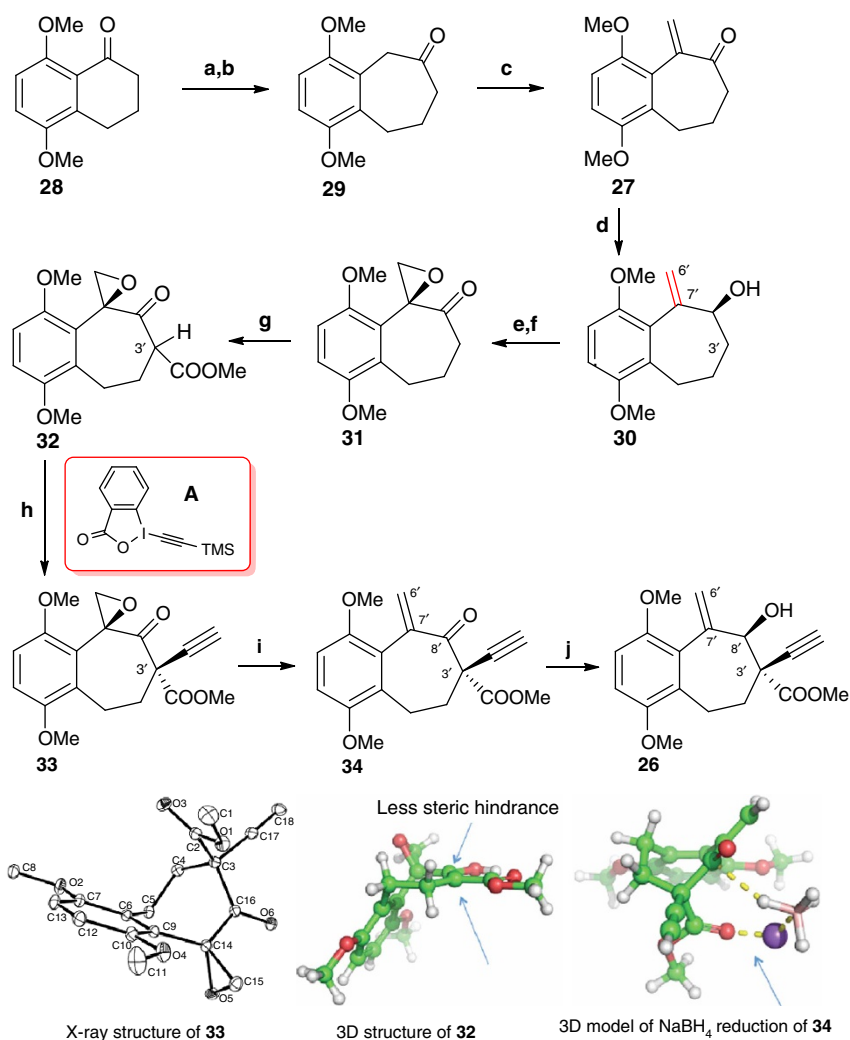
Figure 6 | Synthetic pathways for the construction of intermediate 26. (a) PPh 3 CH 2 Br, THF, KHMDS 0 °C to 25 °C, 98%; (b) Ph(OAc) 2 , p-TSA, MeCN, 0 °C, 95%; (c) Et 3 N · HCl, Et 2 NH, (CH 2 O) n , 1,4-dioxane, 105 °C, 98%; (d) (R)-CBS, BH 3 , THF, -20 °C, 91%, 92% ee; (e) meta-chloroperoxybenzoic acid ( m -CPBA), NaHPO 4 , PhH, 25 °C; (f) Dess-Martin periodinane, NaHCO 3 , DCM, 25 °C, 81% for two steps; (g) LiHMDS, NCCOOMe, THF, -78 °C; (h) tetra- n -butylammonium fluoride, A , THF, -30 °C, 62%; (i) NaI, MeCN, CF 3 COOH, 0 °C, 92%; (j) NaBH 4 , CeCl 3 · 7H 2 O, EtOH, 0 °C, 63%. KHMDS: Potassium bis(trimethylsilyl)amide.
