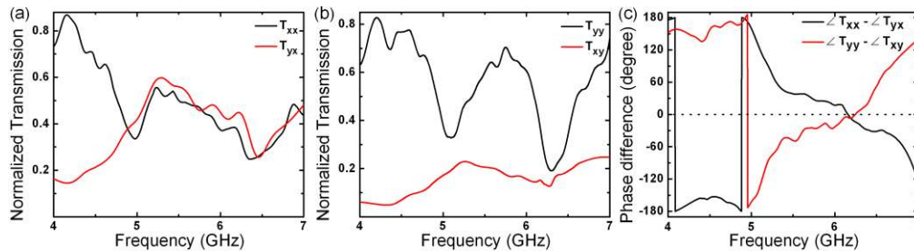
Fig. 4. (a) Experimental magnitudes of T_{xx} and T_{yx} , and (b) T_{xy} and T_{yy} . (c) Mutual phase differences obtained from the experiments.
