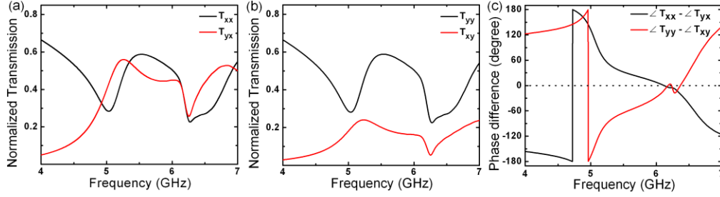
Fig. 2. Magnitudes of the linear transmission coefficients when the CMM is illuminated by (a) x -polarized and (b) y -polarized incident waves. (c) The mutual phase differences between the transmission coefficients.
