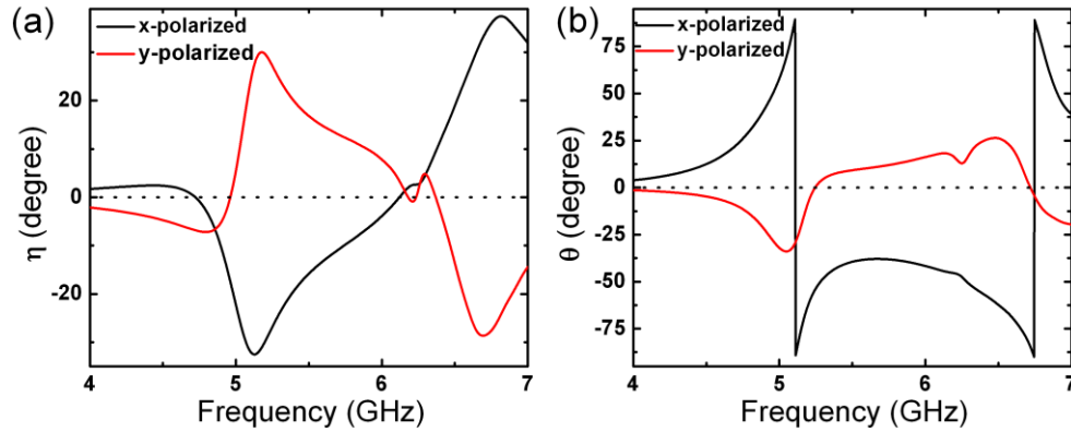
Fig. 3. (a) Ellipticities and (b) polarization azimuth rotation angles of the transmitted waves for x -polarized and y -polarized illumination.
