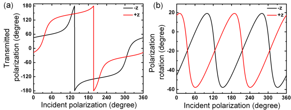
Fig. 6. (a) Polarization angles of the transmitted linearly polarized waves with respect to the polarization angle of the incident wave, at 6.2 GHz, for the -z and +z propagating waves (b) Introduced polarization rotation to the -z and +z propagating waves with respect to the incident polarization angle, at 6.2 GHz.
