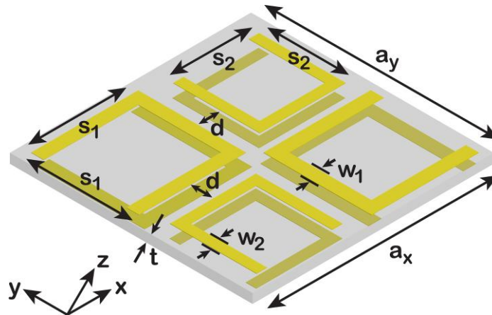
Fig. 1. Geometry of the simulated and fabricated chiral metamaterial unit cell.
