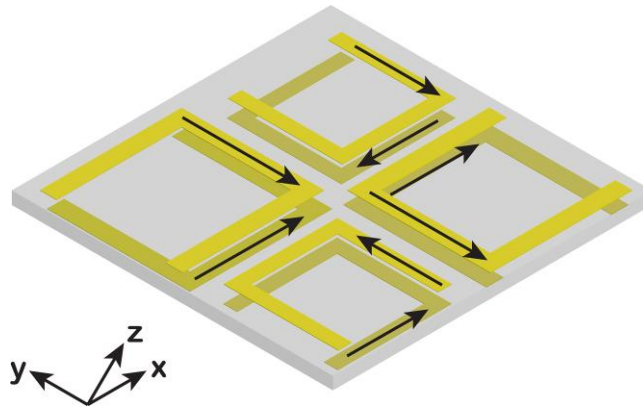
Fig. 7. Directions of the induced surface currents due to x -polarized plane waves propagating in the -z and +z directions at 6.2 GHz.
